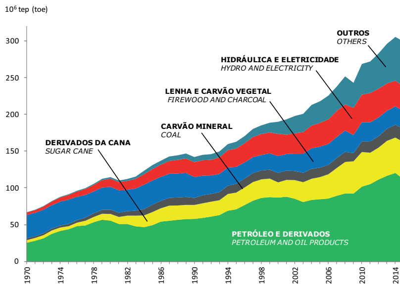
Chart 1.3.a – Domestic Energy Supply
