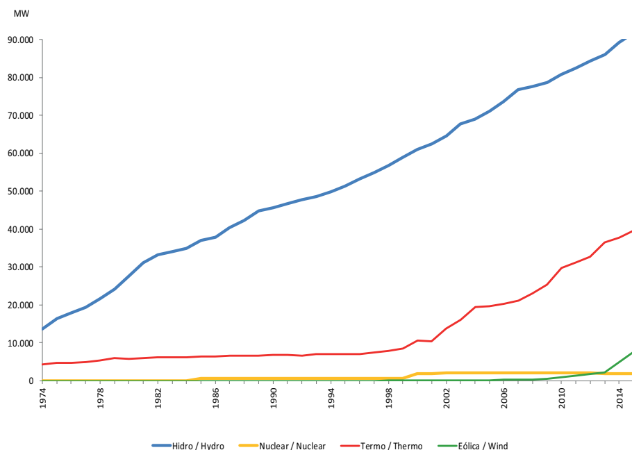
Chart I.1 – Installed Capacity Of Electric Energy Generation
