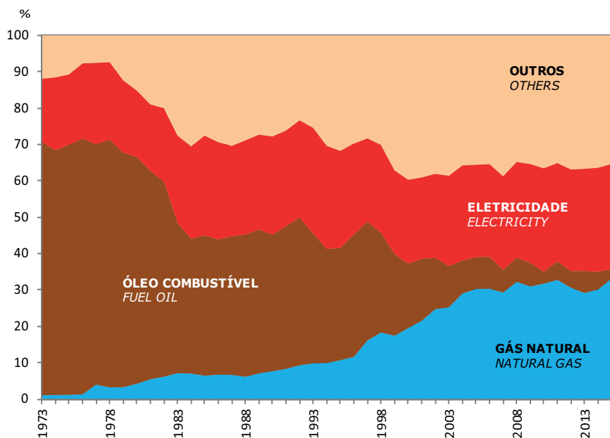
Chart 3.8 – Chemical Sector Energy Consumption
