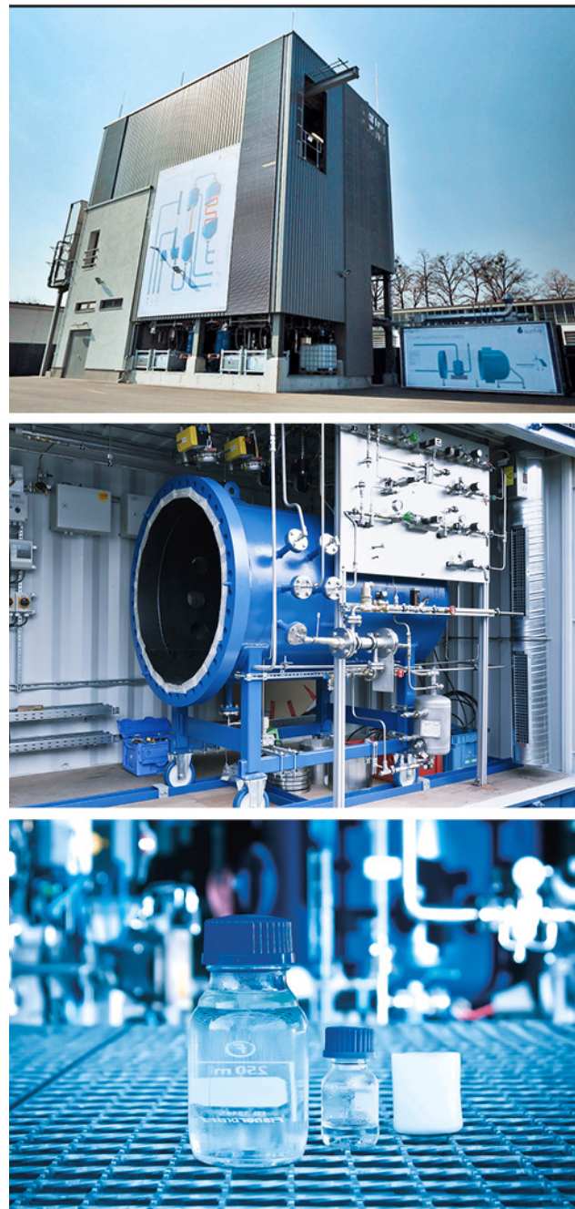
Sunfire PtL demonstration plant (top) using high-temperature electrolysis (middle) for the production of Fischer-Tropsch crude (bottom)
