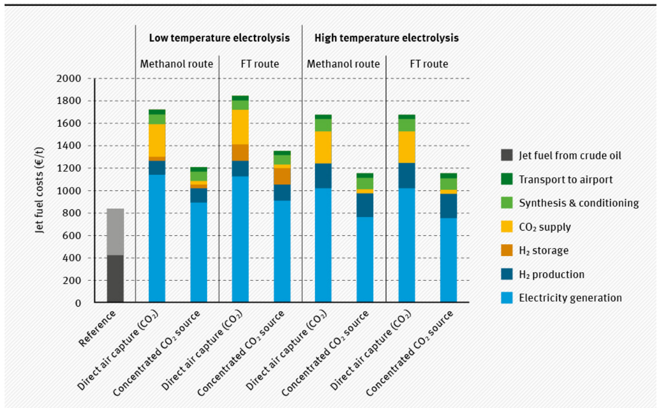
Jet fuel costs projected for future PtL plants in 2050 (jet fuel reference price: 42–95 US$/bbl; renewable electricity costs: 40 €/MWh e ; equivalent full-load period: 3750 h eq /yr)
