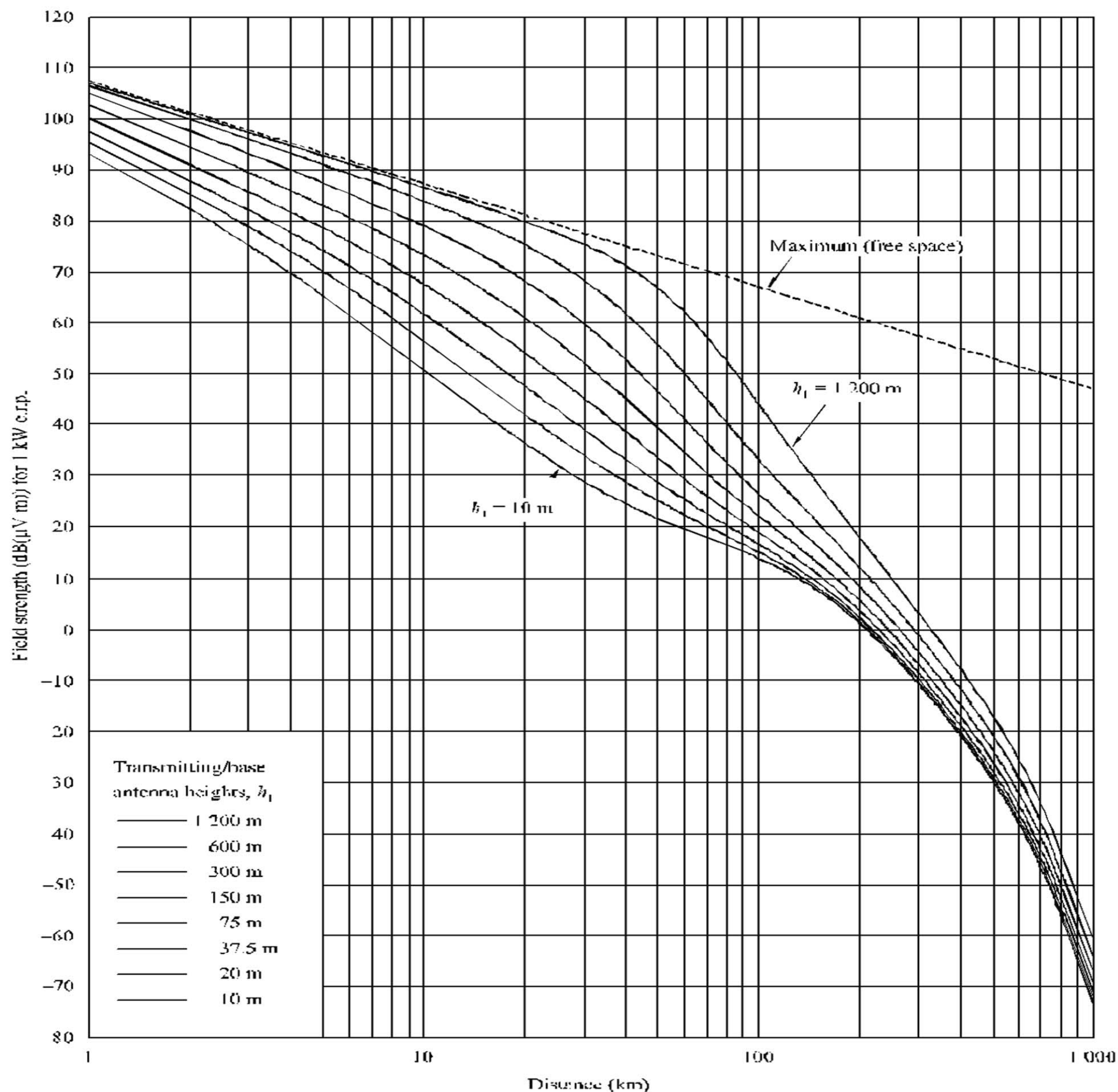
FIGURE 10 600 MHz, land path, 10% time
