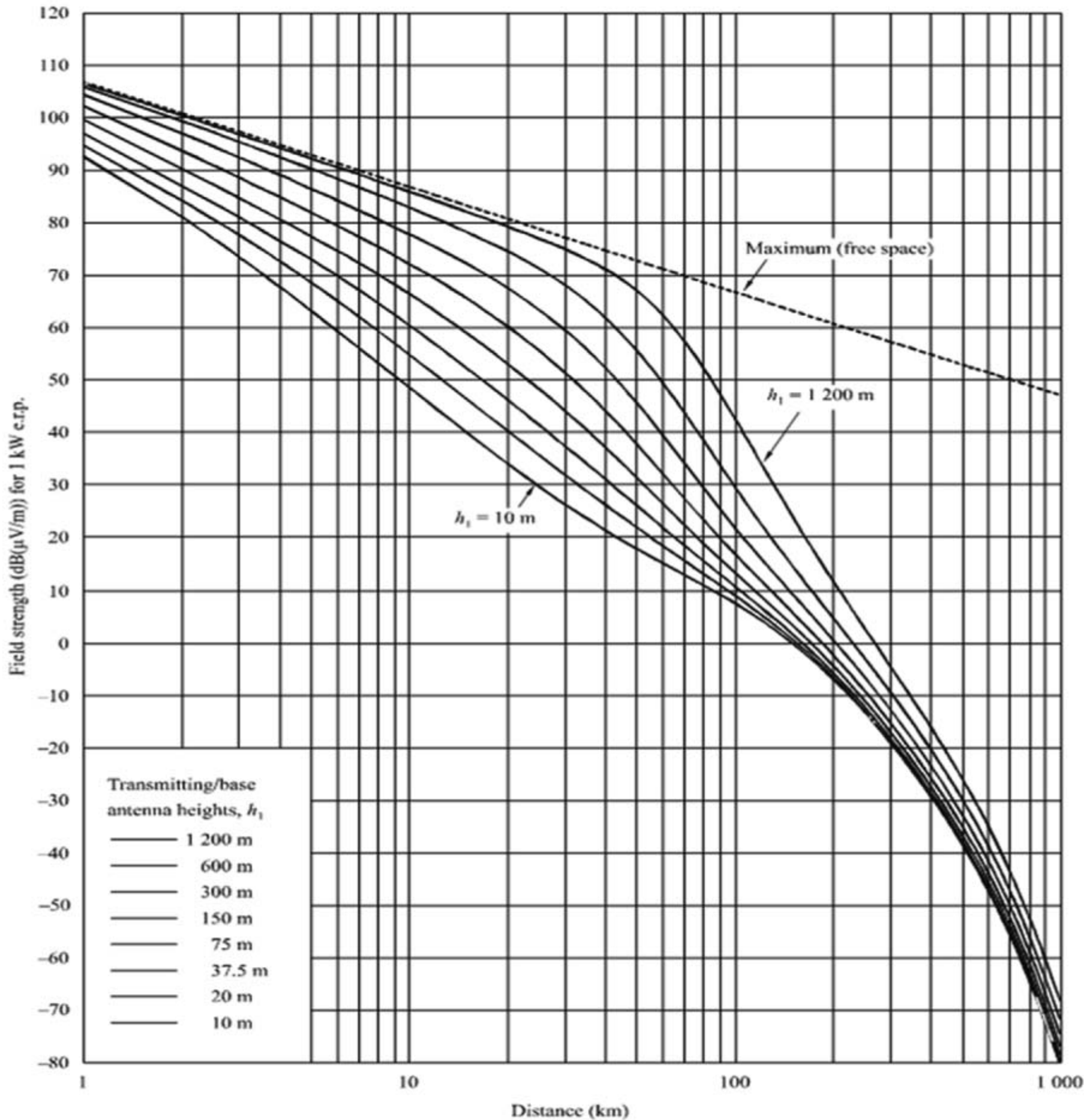
FIGURE 9 600 MHz, land path, 50% time
