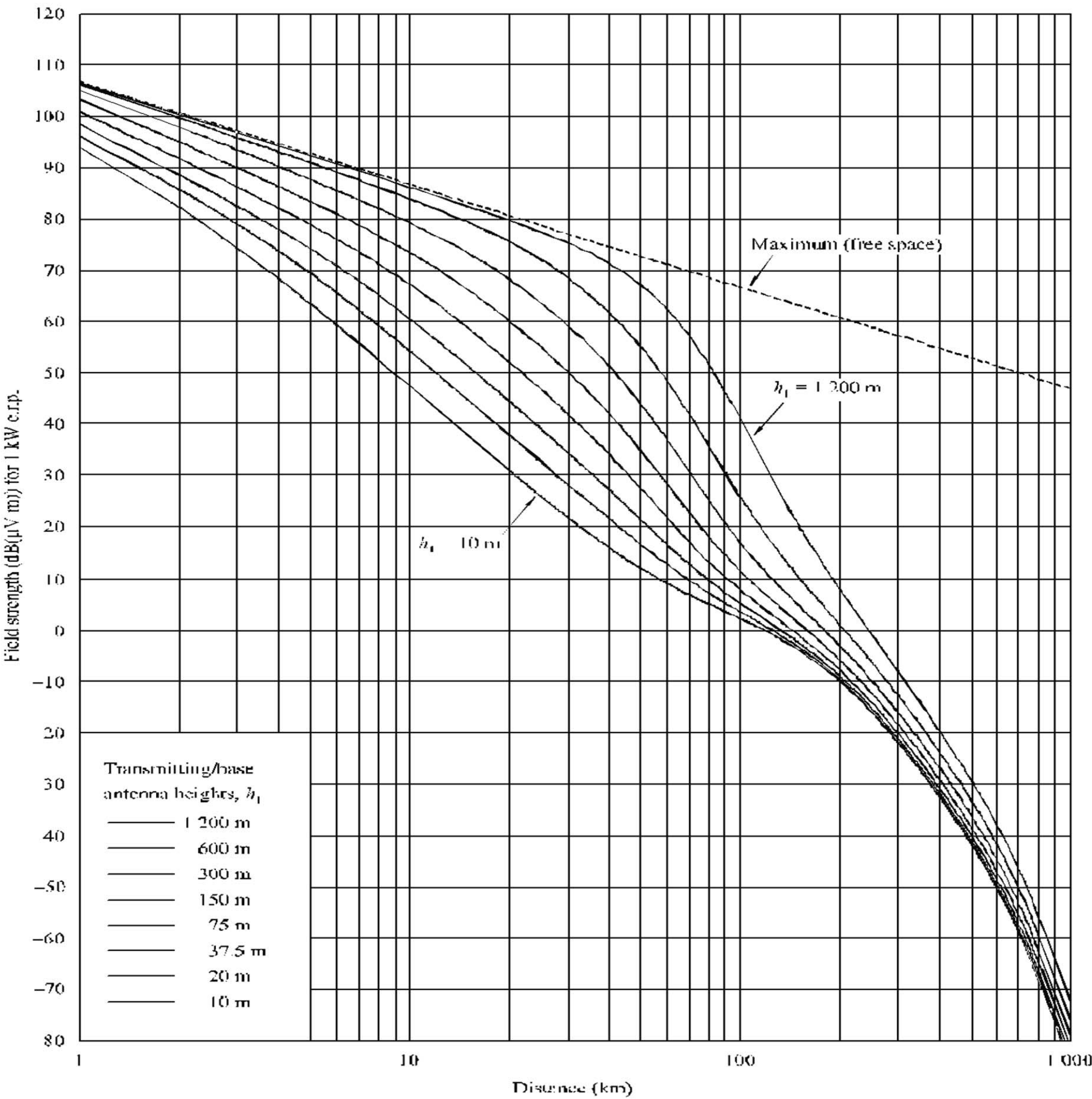
FIGURE 17 2 000 MHz, land path, 50% time
