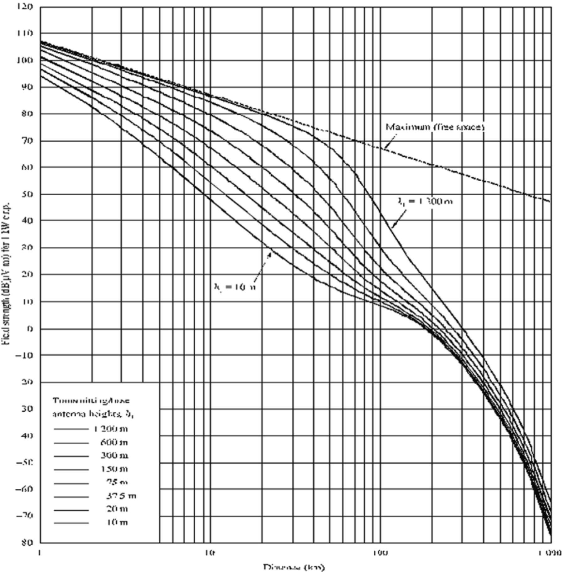
FIGURE 18 2 000 MHz land path, 10% time
