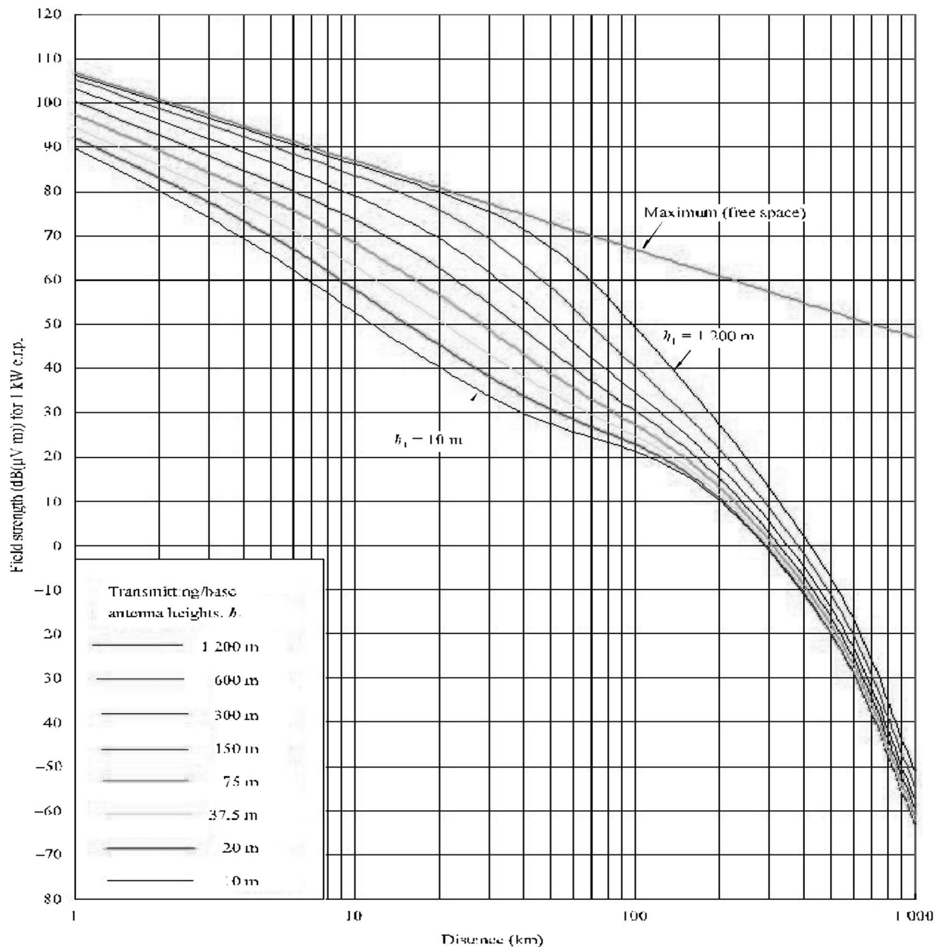
FIGURE 2 100 MHz, land path, 10% time
