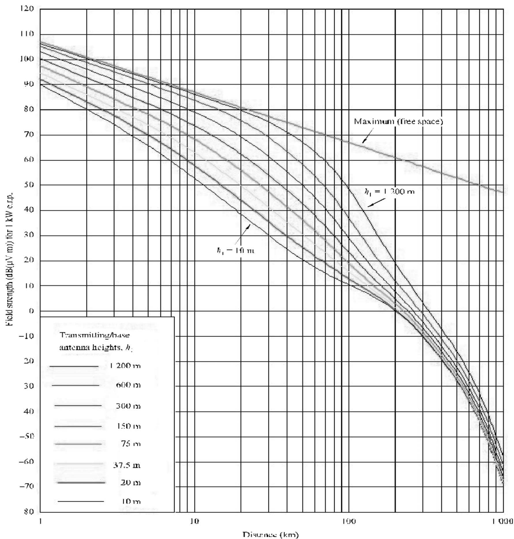
FIGURE 1 100 MHz, land path, 50% time
