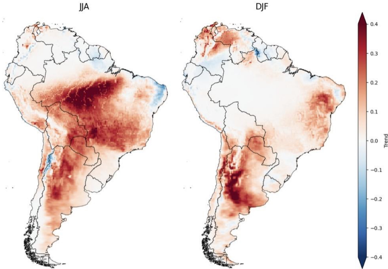
Figure 3. Fire Weather Index (FWI) trends in South America over 1980-2021, covering the austral summer (DJF) and winter (JJA). Trends were estimated by simple linear regression (using ordinary least squares) and colours represent the resulting slope. Data source: ECMWF's ERA5 FWI estimates .
