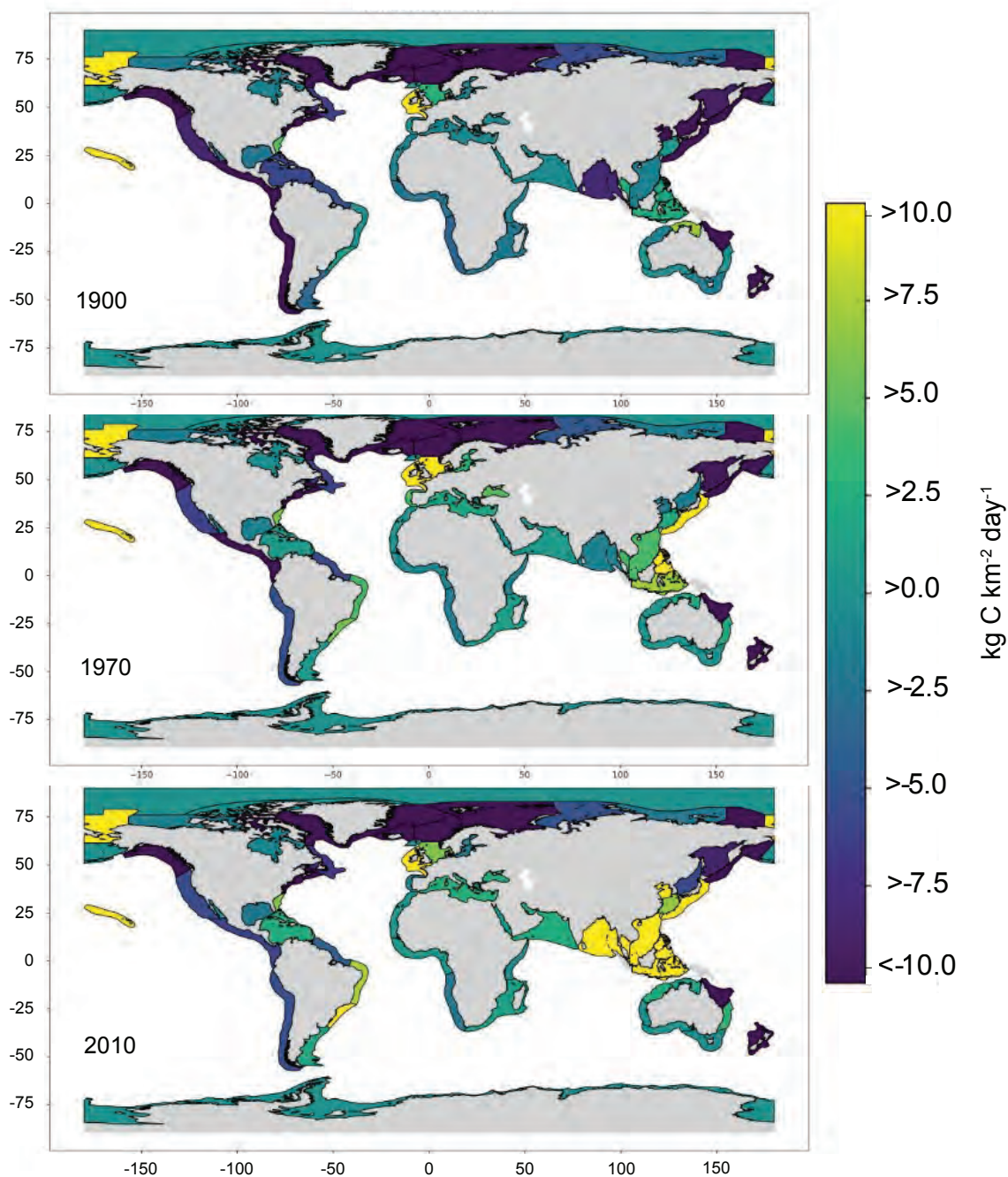
Figure 2. Indicator of Coastal Eutrophication Potential (ICEP) values for coastal river inputs aggregated to the scale of LMEs for years 1900 (top), 1970 (middle) and 2010 (bottom). ICEP is calculated as the excess of N or P over the requirement of diatoms based on the Redfield ratio and is expressed as the potential growth of non-diatom species in kg C-equivalents per \text{km}^2 per day (Beusen and Bouwman, 2022; Liu et al., 2020). High values suggest a high potential for the formation of HABs. Pronounced increases in ICEP have occurred over time, particularly in South and Southeast Asia and off the coast of eastern South America. Source: Authors' compilation.
