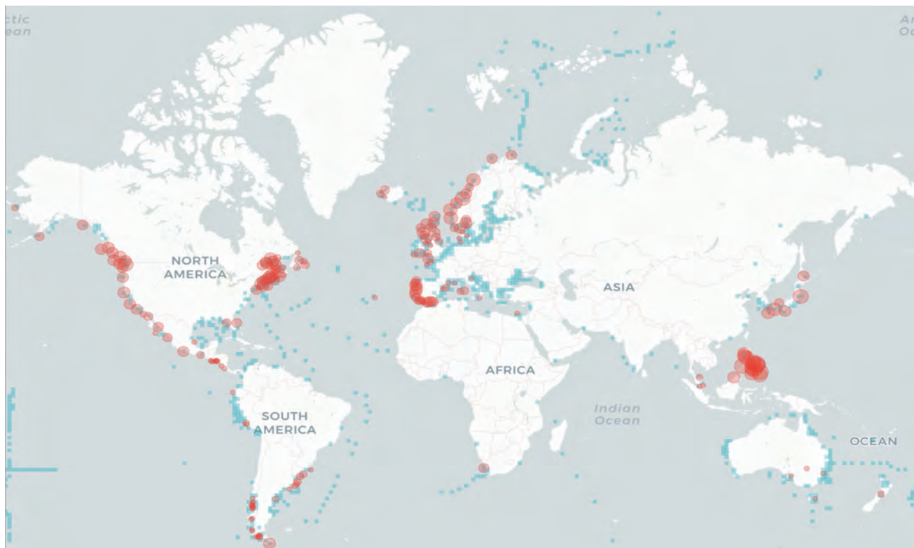
Figure 24. World map of distribution events associated with paralytic shellfish toxins (red) combined with that of the occurrence of Alexandrium causative organisms (blue). The larger the bubbles, the more events were observed in a locality. Source: Based on data obtained from the HAIS Data Portal https://data.hais.ioc-unesco.org/ .
