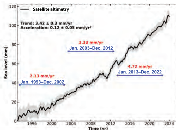
Figure 19. Global mean sea level rise from satellite altimetry from January 1993 to December 2023 (black curve). The shaded area represents the uncertainty. The blue horizontal lines indicate successive global mean sea level trends. Altimetry data from AVISO 8 . Source: LEGOS.
