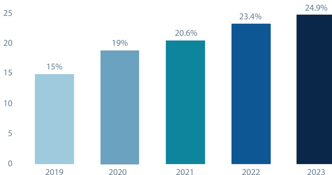
Figure 32. Percentage of seafloor mapped within the GEBCO grid per year. Source: Adapted from Seabed 2030 Global Center and Stockholm University.
