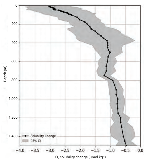
Figure 9. Global mean O_2 solubility content decrease as a function of depth after 60 years (Garcia et al., 2024). Source: World Ocean Database.
