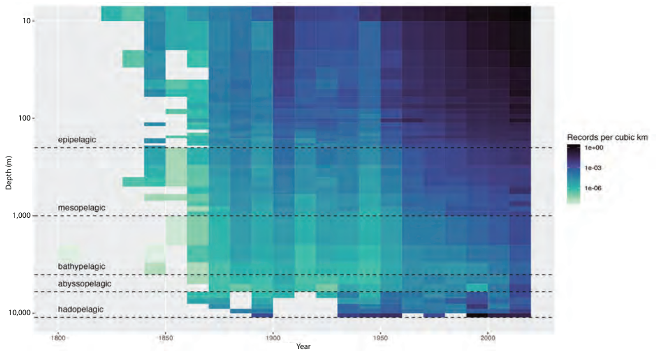
Figure 27. Number of OBIS records per km 3 of ocean volume, over time and per depth zone, clearly illustrating the trend of going deeper. Source: OBIS.
