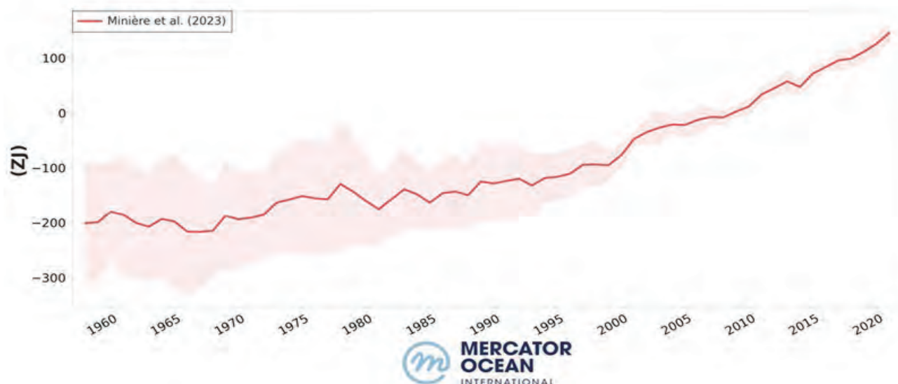
Figure 6. Global mean ocean heat content from 1960–2023 (in ZJ) for the upper 2,000 m depth as derived as an ensemble mean approach considering several subsurface temperature products and its uncertainty (shaded). Source: Minière et al. (2023).
