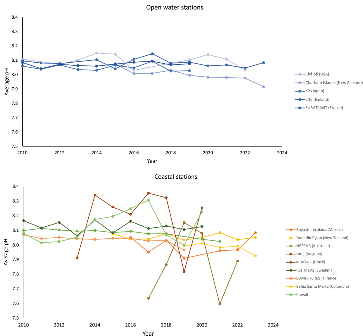
Figure 5. Variations in the annual average pH values from a suite of representative sampling stations in open and coastal waters. Data from IOC/UNESCO, SDG14.3.1 ocean acidification reporting. Notes: Open water stations: Chá bă – USA, Pacific Ocean (data from 2010–2022); Chatham Island – New Zealand, South Pacific Ocean (data from 2015–2023); K2 – Japan, North Pacific Ocean (data from 2010–2019); LN6 – Iceland, Iceland Sea, North Atlantic Ocean (data from 2010–2023); SURATLANT – France, Atlantic Ocean (data from 2010–2019). Coastal water stations: Boya de recalada – Mexico, Pacific Ocean (data from 2016–2023); Dunedin Pylon – New Zealand (data from 2015–2023); NRSPHB – Australia, National Reference Station Port Hacking station (data from 2010–2021); W03 – Belgium, Scheldt Estuary (data from 2013–2020); # BrOA1 – Brazil, Reference Station (data from 2017–2022); REF M1V1 – Sweden, Reference Station (data from 2010–2020); SOMLIT-BREST – France, Celtic Sea (data from 2010–2019); Bahía Santa Marta – Colombia, Caribbean Sea (data from 2019–2023); Kuwait – Kuwait Bay (data from 2010–2020). Source: IOC-UNESCO.
