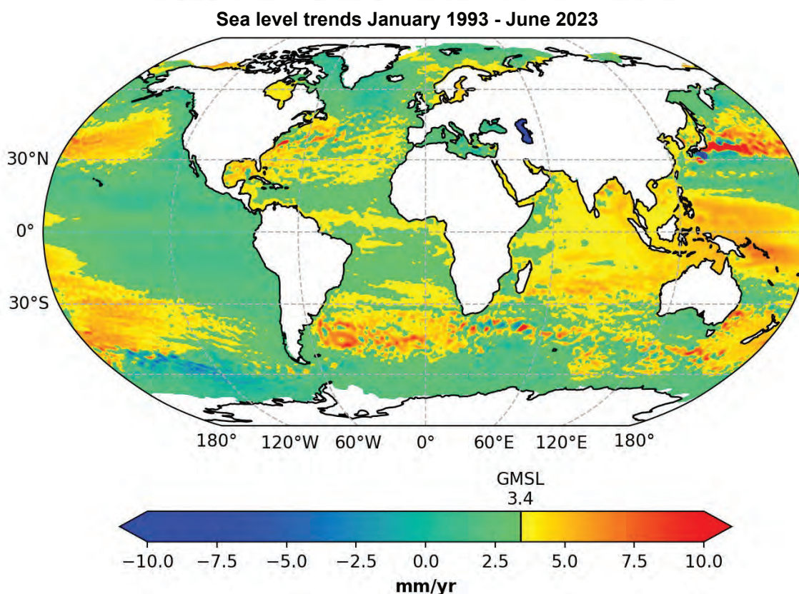
Figure 20. Regional sea level trends ( \text{mm yr}^{-1} ) from January 1993 to June 2023, based on multimission satellite altimetry. The colour transition from green to yellow corresponds to the global mean sea level (GMSL) rise. Source: Altimetry data from the Copernicus Climate Change Service 9
