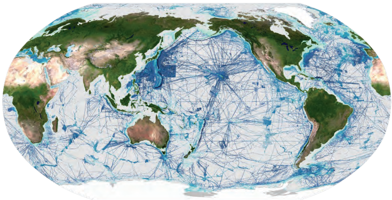
Figure 31. The areas shown in shades of blue are the regions of the GEBCO_2023 Grid that are considered mapped, i.e. based on measured data rather than prediction/interpolation. Source: Seabed 2030 Global Center.
