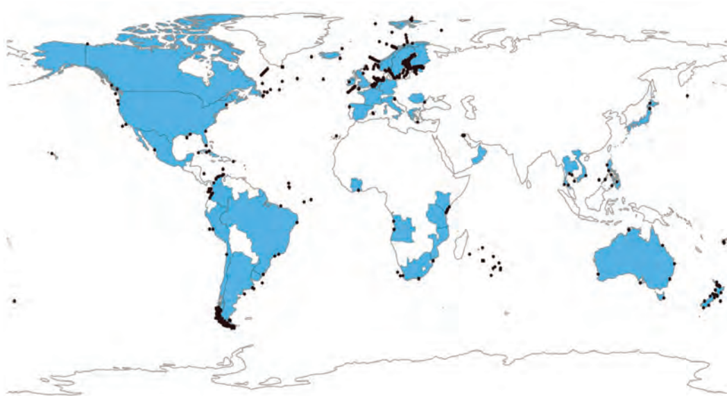
Figure 4. Map illustrating surface ocean carbonate chemistry measurement locations received by the IOC for SDG 14.3.1 ocean acidification reporting. Blue: countries whose data was reported in accordance with the SDG 14.3.1 Indicator Methodology. Black dots: location of sampling stations from which data was collected (539 stations in 2023). Source: IOC-UNESCO.
