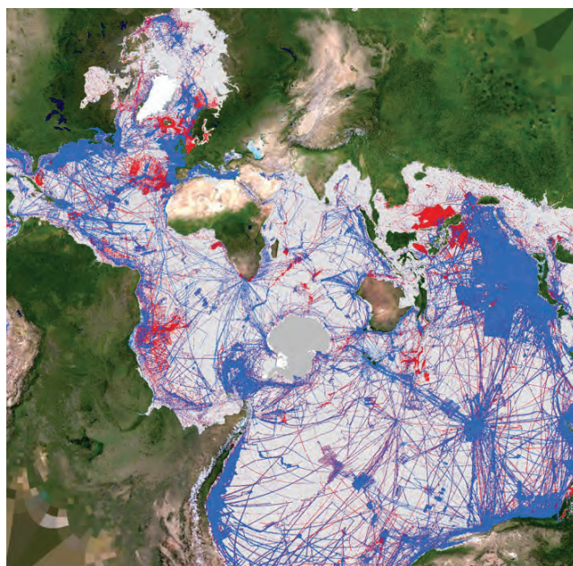
Figure 33. The blue areas show what regions are considered mapped in the 2021 GEBCO grid, and the areas in red show the increase in coverage recorded in 2023. Source: Seabed 2030 Global Center.
