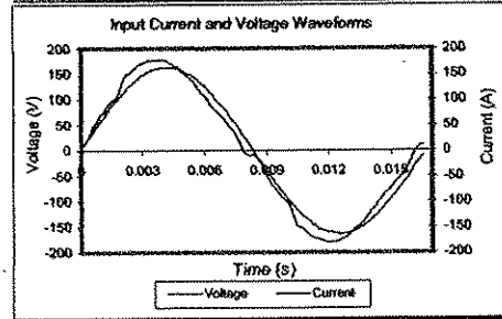
Input AC Current Waveform (THD = 7.98%, 50% Load)
