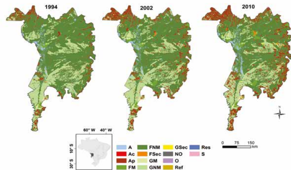
FIGURE A1.13 Land use / cover maps of the Pantanal biome for 1994, 2002, and 2010
