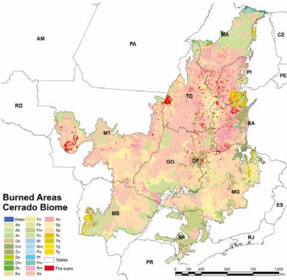
FIGURE A2.2 Distribution of fire scars mapped in 2010 in the Cerrado biome
