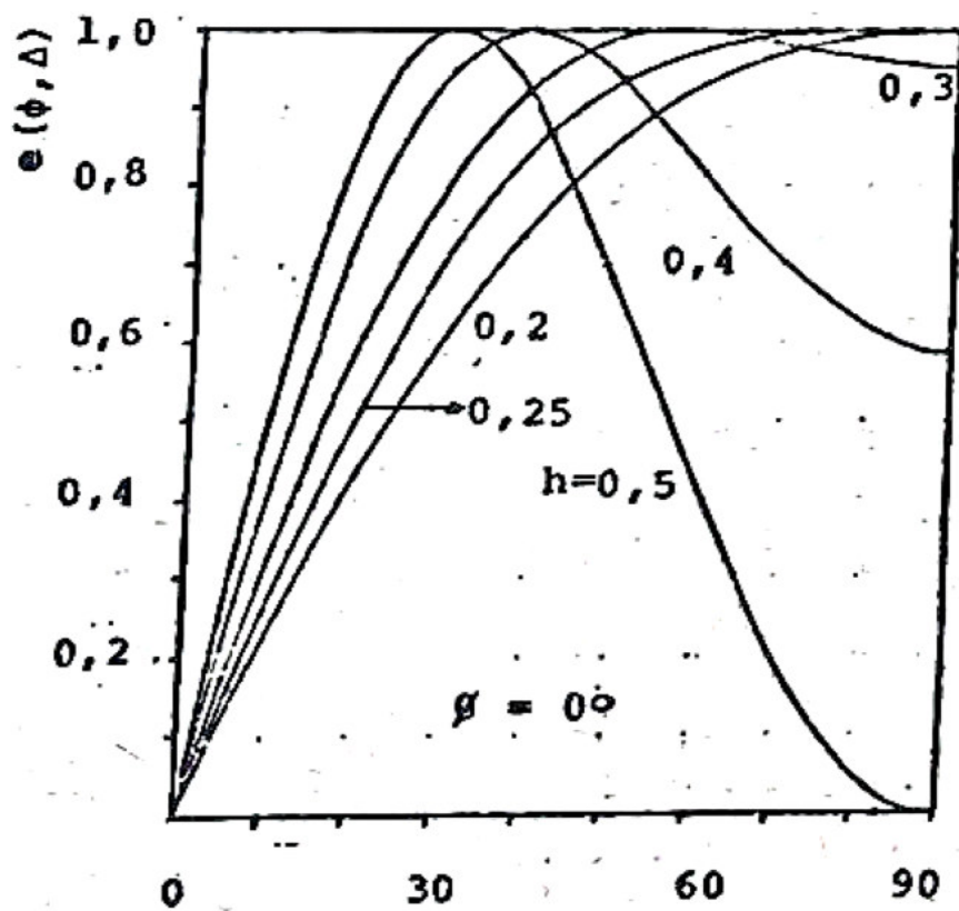
Fig. VII.8 Diagrama Vertical. Antena H 1/\lambda
