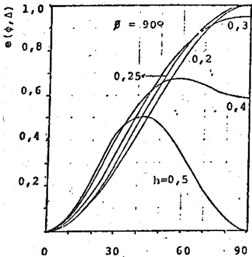
Fig. VII.9 Diagrama Vertical. Antena H 1/\lambda
