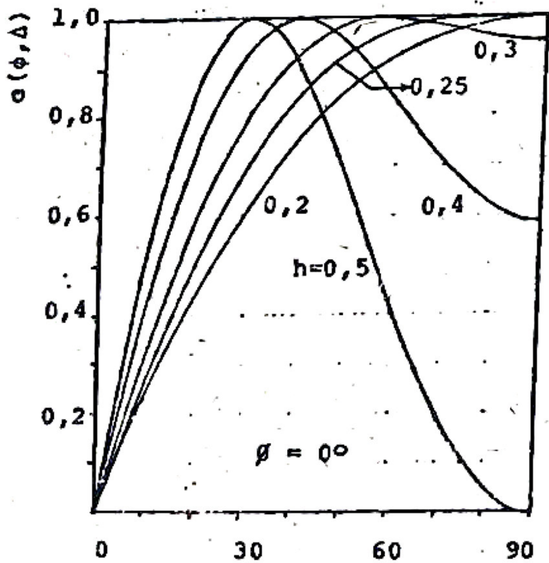
Fig. VII.10 Diagrama Vertical. Antena H \frac{2}{1/\lambda}
