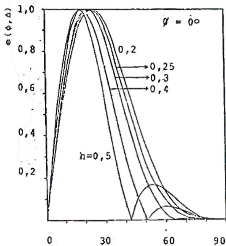
Fig. VII.24 Diagrama Vertical. Antena HR 1/2/\lambda . Plano refletor infinito, s=0,25\lambda .
