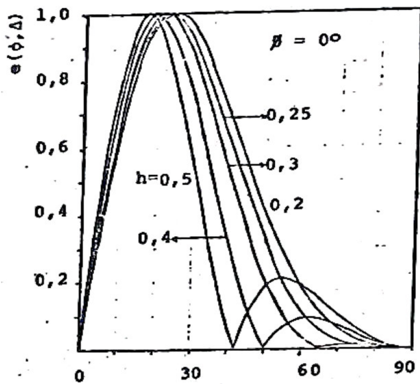
Fig. VII.12 Diagrama Vertical. Antena H 2/1/\lambda .
