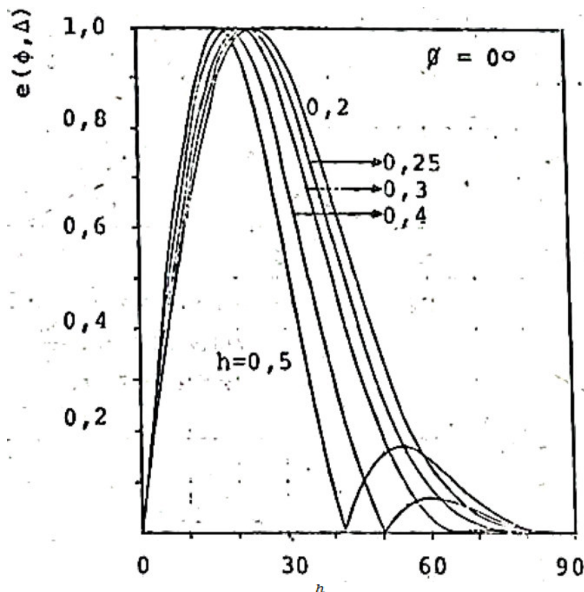
Fig. VII.25 Diagrama Vertical. Antena HR 2/2/\lambda . Plano refletor infinito, s=0,25\lambda .
