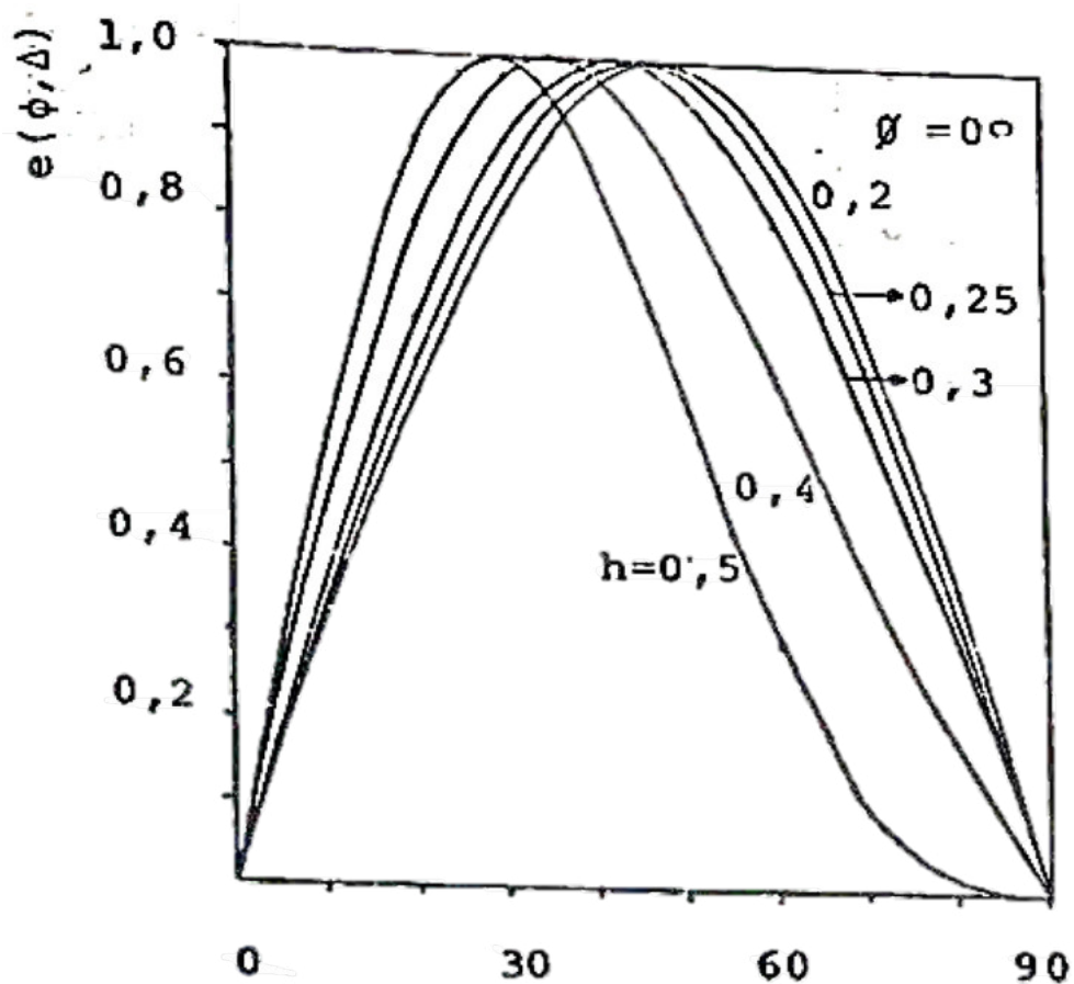
Fig. VII.23 Diagrama Vertical. Antena HR 2/1/\lambda . Plano refletor infinito, s=0,25\lambda .
