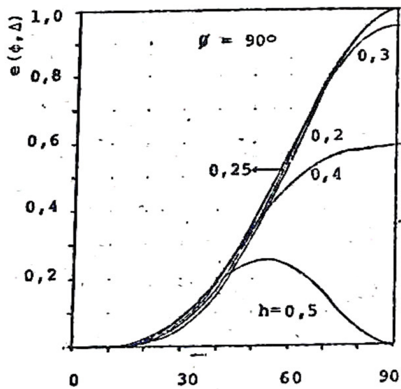
Fig. VII.11 Diagrama Vertical. Antena H 2/1/\lambda .
