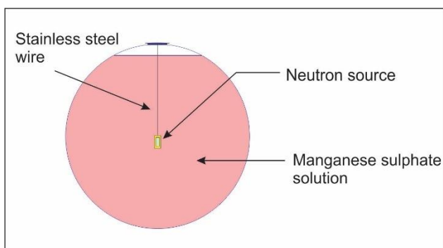
Figure VI.2 - Scheme of a static manganese sulfate bath
