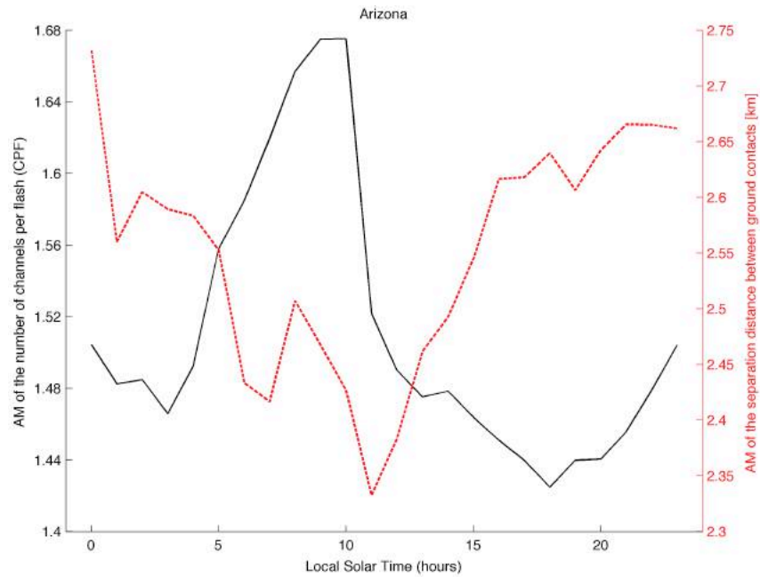
Figure 8.5 – Hourly plots of the AM of the number of channels per flash (CPF) and the separation distance between ground contacts in the Arizona domain.
