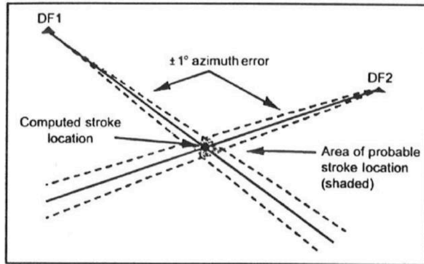
Figure 3.6 – Return stroke location from two magnetic direction finders.
