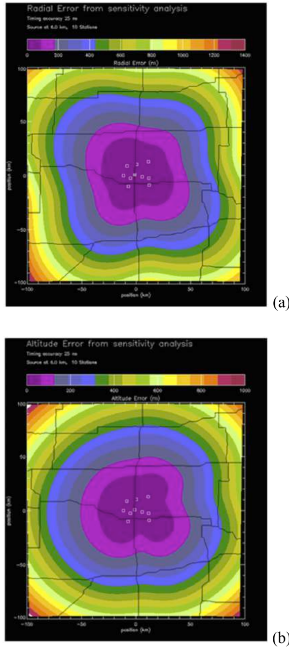
Figure 3.16 – Estimated location accuracy of the LMA used during the KSWFP.
