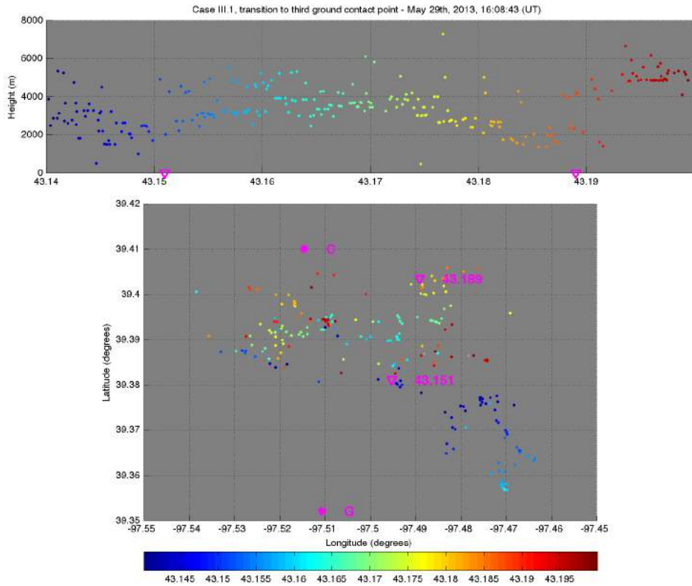
Figure 6.28 – LMA plot of the initiation of the third stroke (NGC) of Case III.1.
