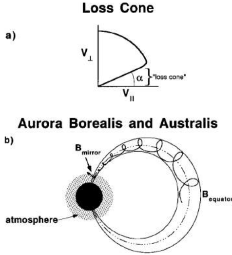
Figure 3.7 - Loss cone.
