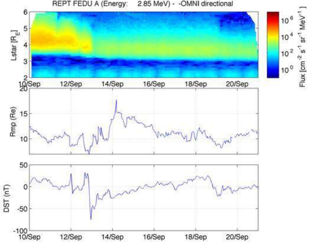
Figure 2.6 - Relativistic Electron flux dropout.
