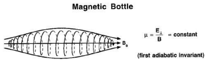
Figure 3.6 - Gyro and bounce motion.
