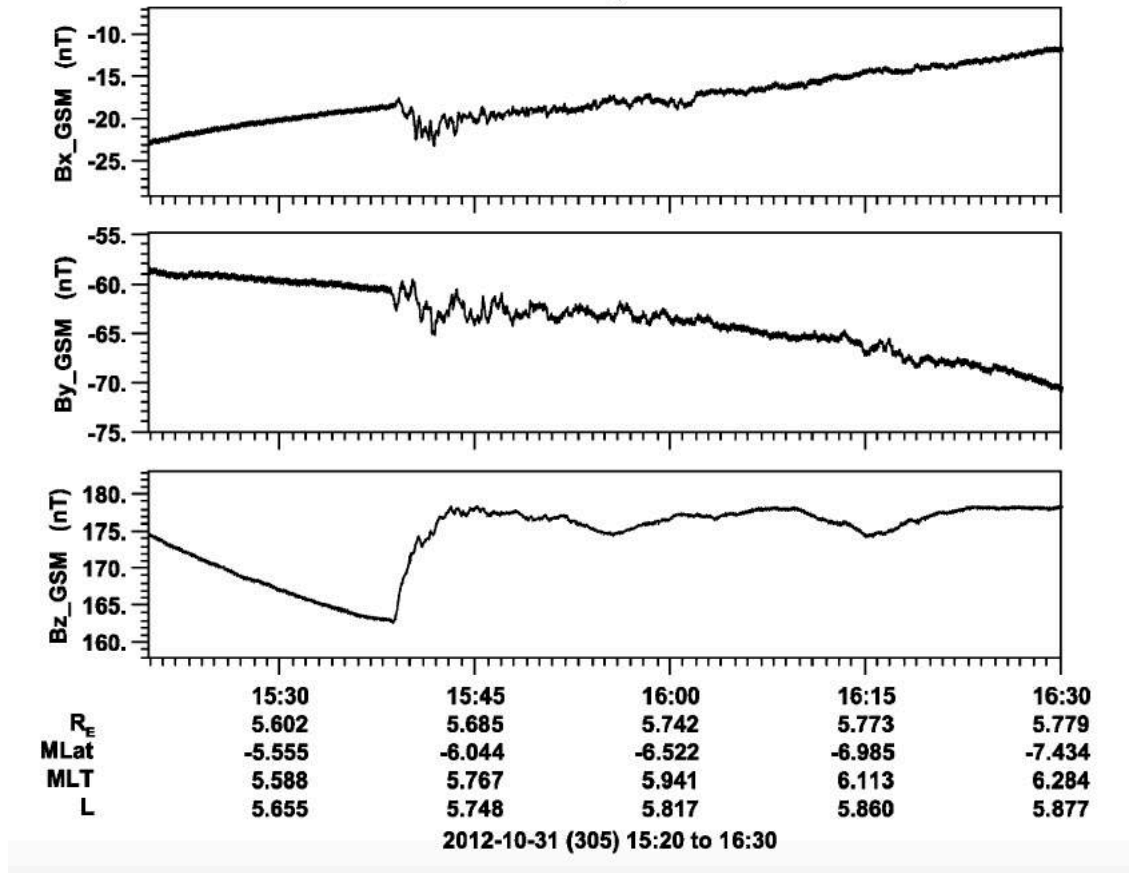
Figure 4.1 - RBSPA/EMFISIS Magnetometer vector.
