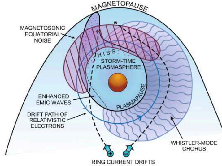
Figure 3.2 - Schematic illustration of waves in the inner magnetosphere
