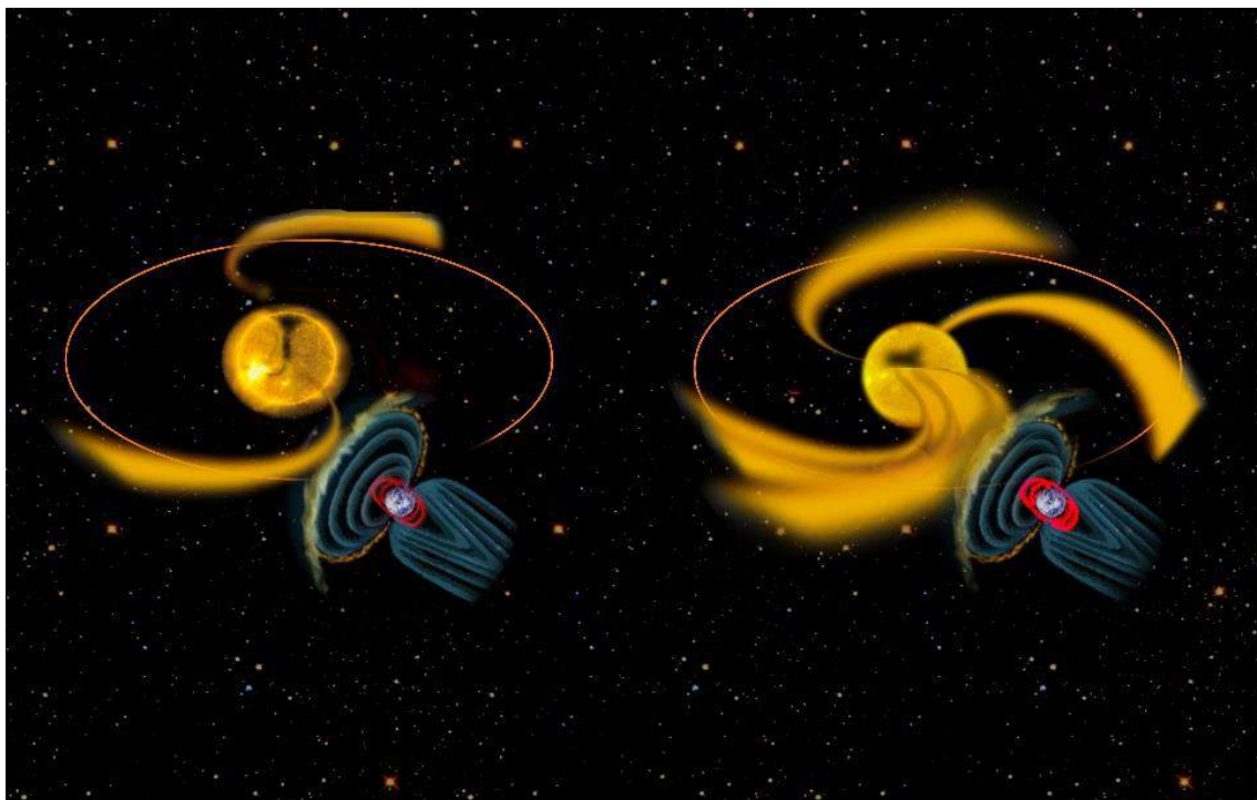
Artist's rendition of both the slow (left) and fast (right) solar wind SOURCE: Gibson et al. (2009) .
