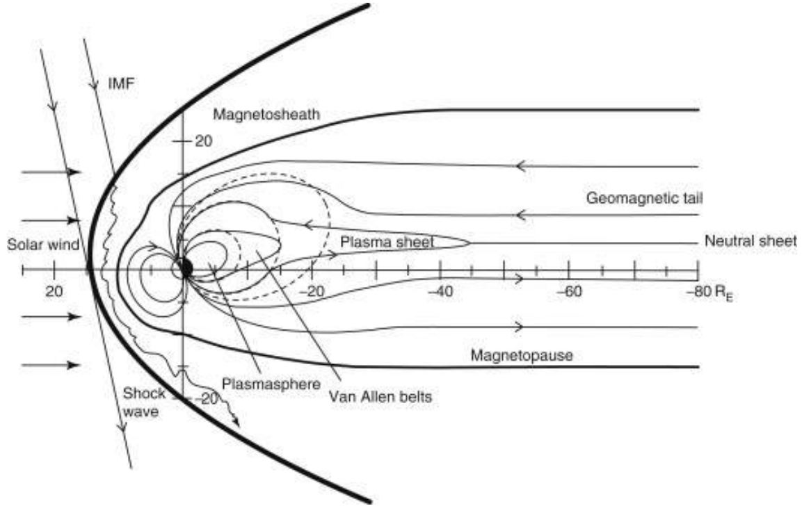
Figure 2.3 - Earth's Magnetosphere.
