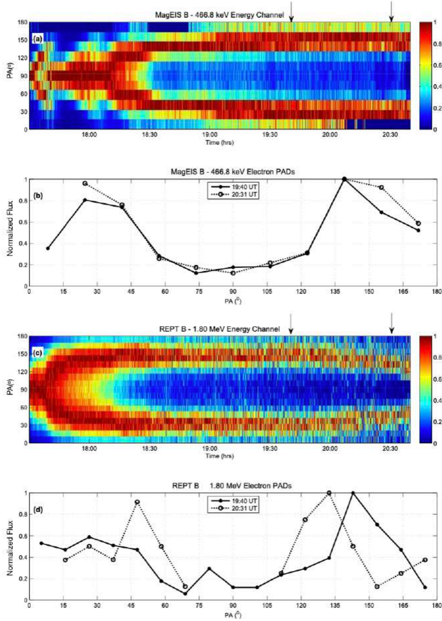
Figure 5.12 - PAD at different energy levels from the REPT and MagEIS.
