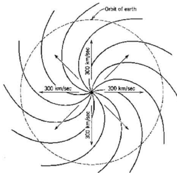
Figure 2.1 - The interplanetary magnetic field.
