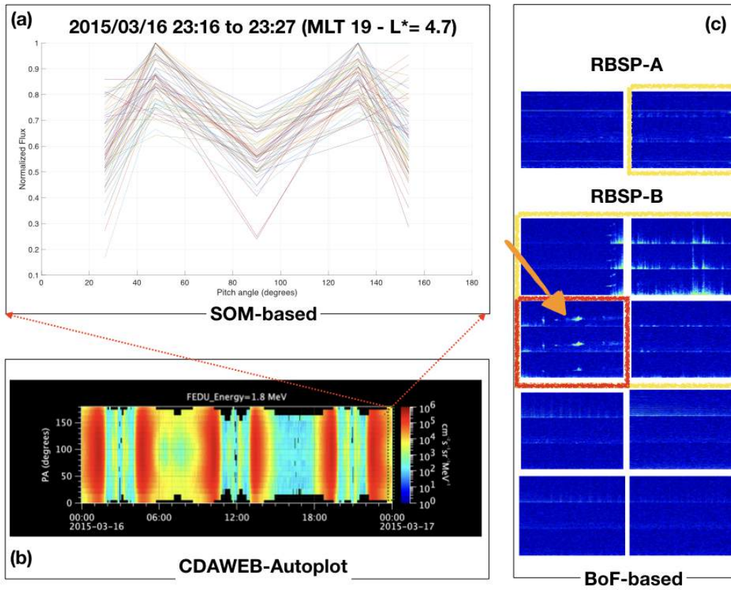
Figure 7.6 - Day before St Patrick storm event.
