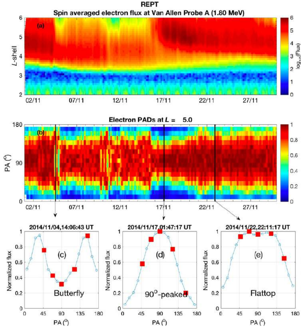
Figure 7.1 - RBSP-A Electron flux and PADs.
