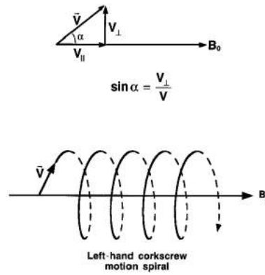
Figure 3.5 - Pitch angle
