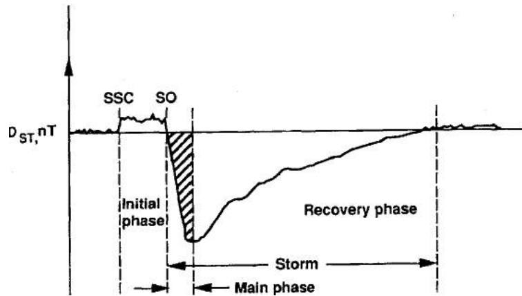
Figure 2.5 - Dst index during a geomagnetic storm.
