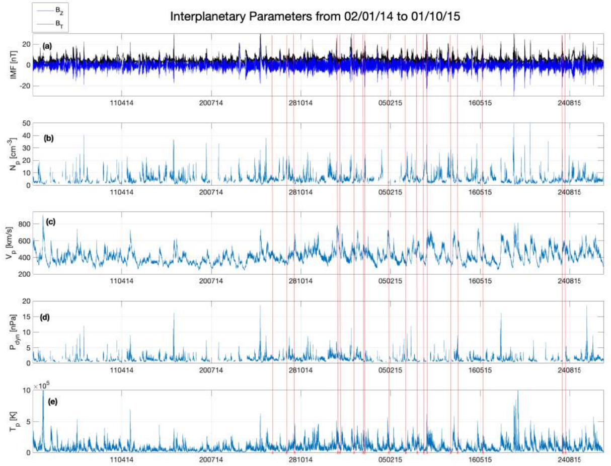
Figure 7.5 - Interplanetary parameter
