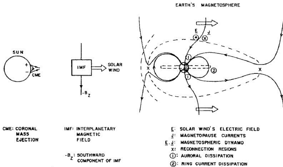
Figure 2.4 - Solar-Earth's magnetic field coupling.
