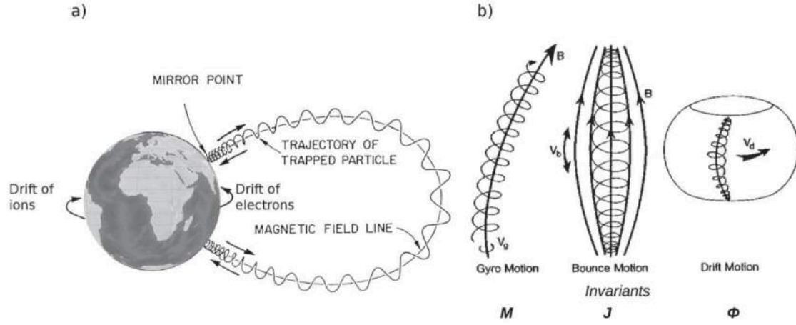
Figure 3.1 - The magnetic trapped charged particle motion.
