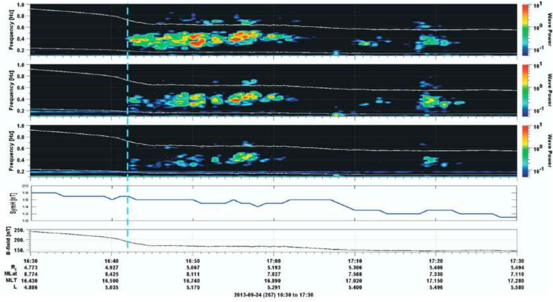
Figure 3.12 - EMIC wave spectrogram.
