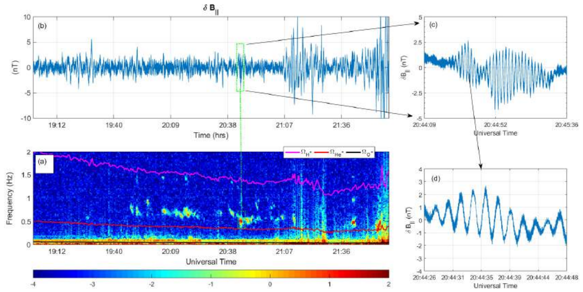
Figure 5.11 - Occurrence of EMIC waves observed by Van Allen Probe B.
