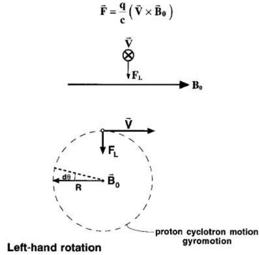
Figure 3.4 - The Lorentz force acting in a proton in a uniform magnetic field.
