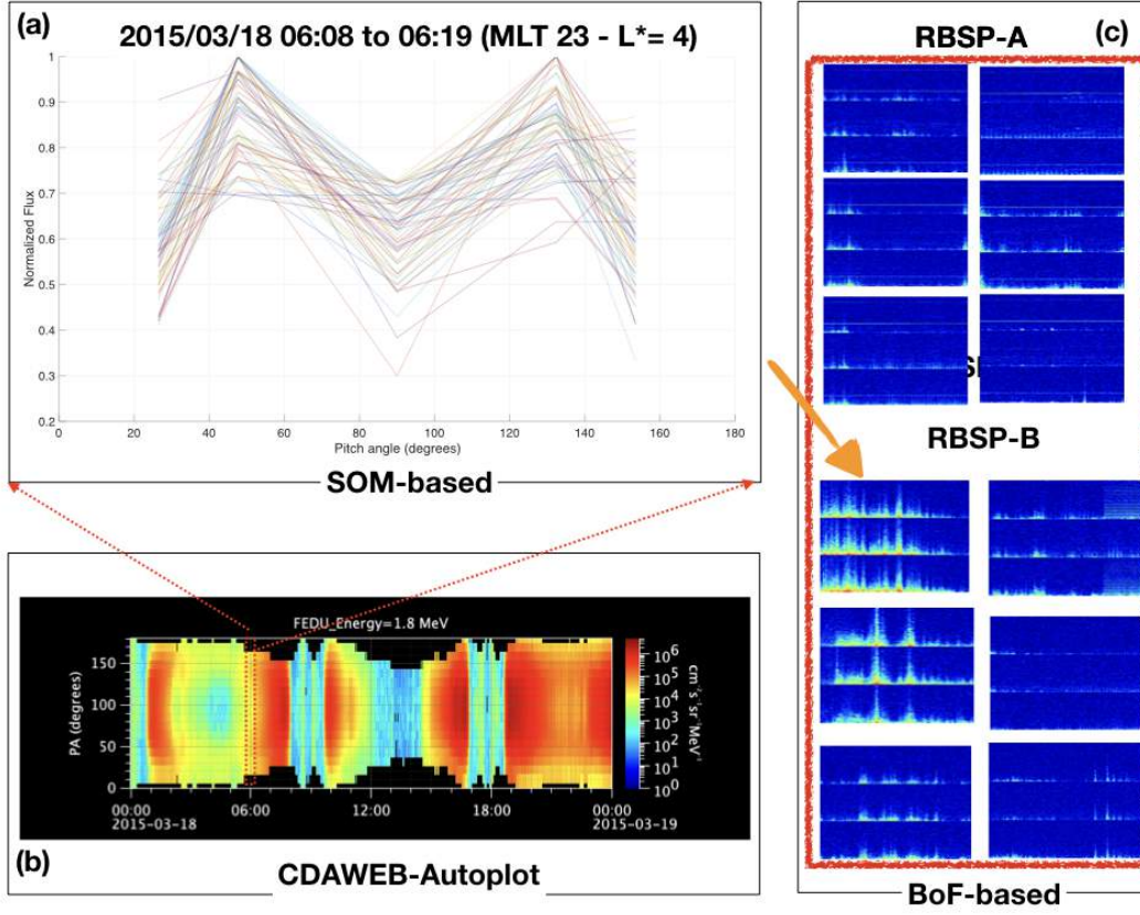
(a) SOM-based classification shown the persistent unusual butterfly PAD shape on March 18, 2015 after 06:08 UT. Van Allen Probe A was in MLT 23 and L-star \sim 4 . (b) The relativistic electron at 1.8 MeV channel shown the pitch angle distribution during one day. (c) BoF technique classified 12 ( 6 by RBSP-A and 6 by RBSP-B ) images as EMIC classes. All of them (red box) presented clear EMIC-like wave signature (orange arrow).
