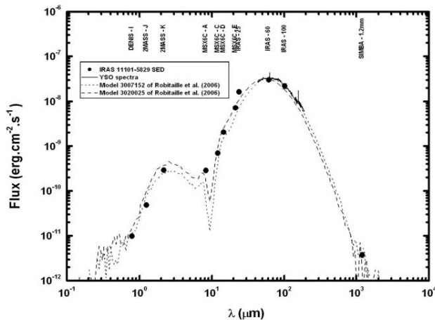
FIG. 10.—SED of IRAS 11101–5829. The observational data are from the following resources: DENIS, VizieR Online Data Catalog, B/denis (N. Epchtein et al., 2005); 2MASS, Cutri et al. (2003); MSX, VizieR Online Data Catalog, 5114 (M. P. Egan et al., 2003); IRAS , Beichman et al. (1988); SIMBA, Hill et al. (2005); ISO , spectrum from the ISO data archive ( http://www.iso.vilspa.esa.es/ida/index.html ). The dotted and dashed lines represent two models from Robitaille et al. (2006; see text for details).
