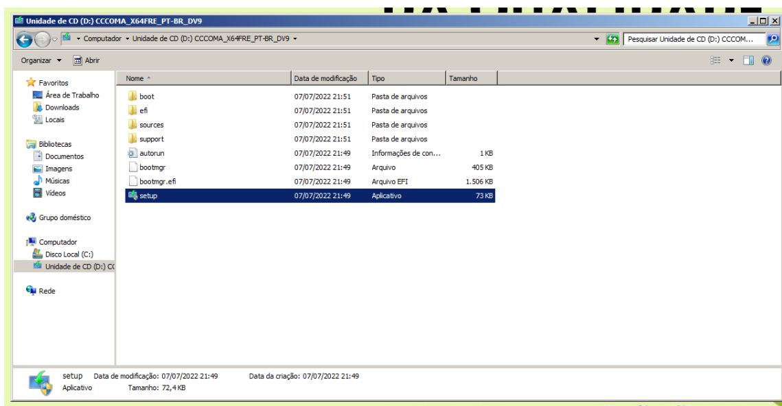
Figura 3 – Executar setup.exe.
