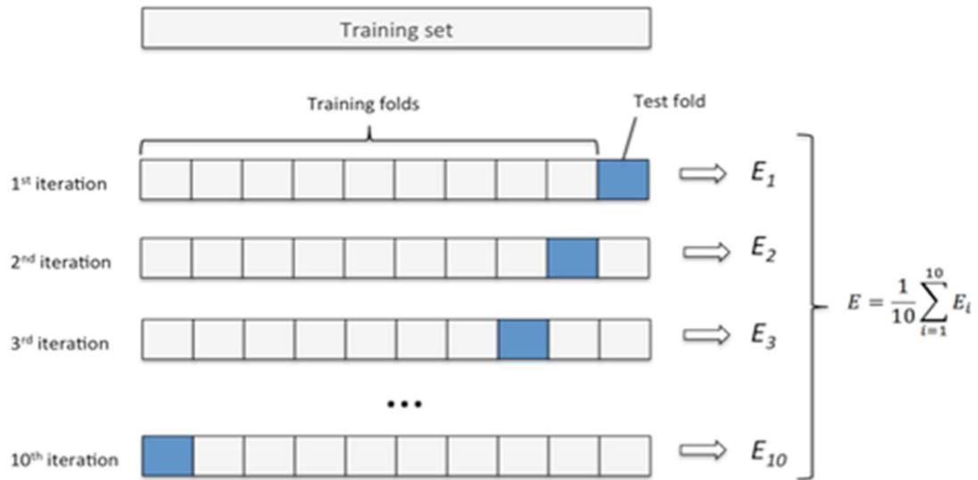
FIGURE 11. K-FOLD CROSS-VALIDATION. SOURCE: SEBASTIANRASCHKA
