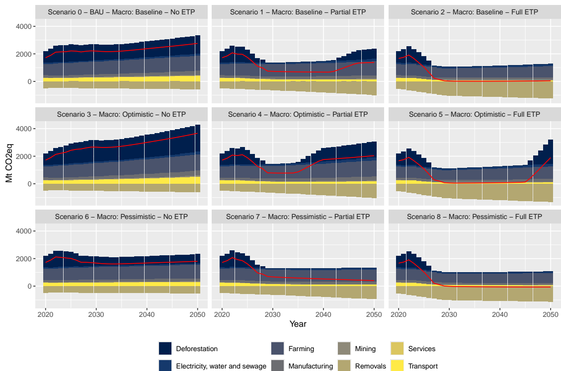
Figure 7: Decomposition of cross-scenarios simulated net emissions of GHG, measured in MtCO 2 eq
