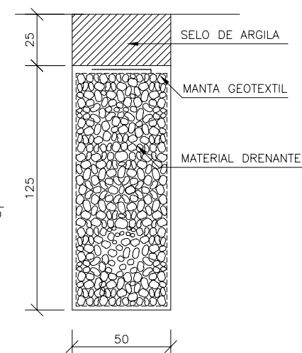
DPS 05 (DRENO CEGO)
