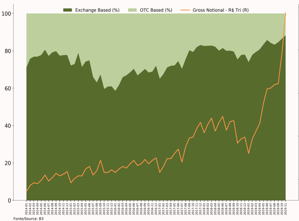
6.4 - Derivatives - Nov/2019
