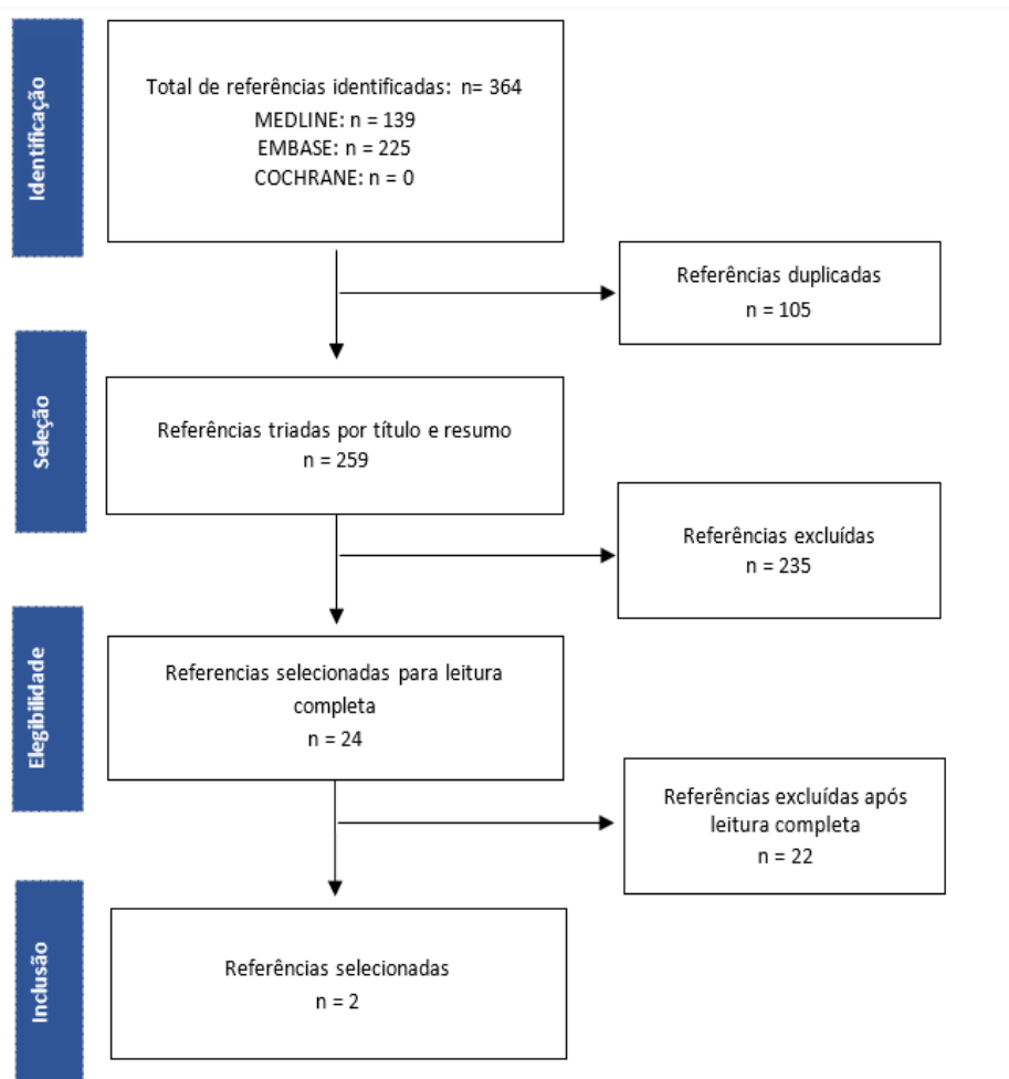
Figura 5. Fluxograma Prisma
