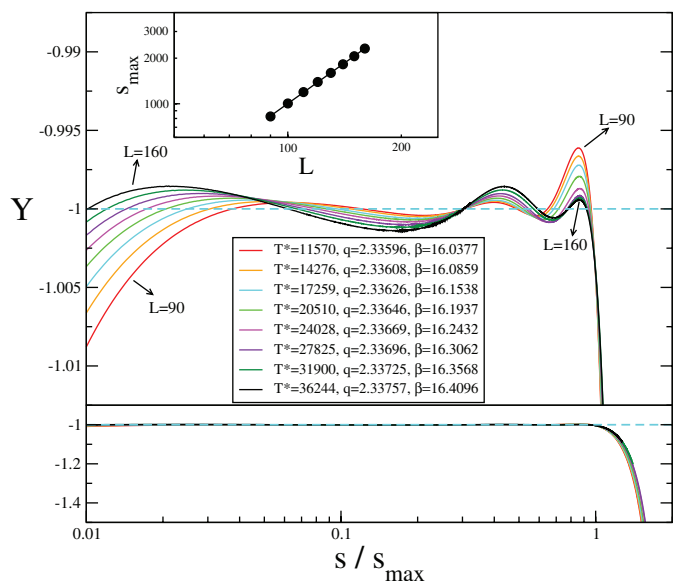
Fig. 4: (Colour on-line) The case a = 1 and p = 5 \cdot 10^{-6} with L values between L = 90 to 160 . The lower panel shows the data collapse when the x -axis is appropriately scaled. The upper panel shows a zoomed region around the Y = -1 line. In the inset the scaling of s_{max} with L is given. The straight line is s_{max} = AL^C with A = 0.2726 and C = 1.7828 .
