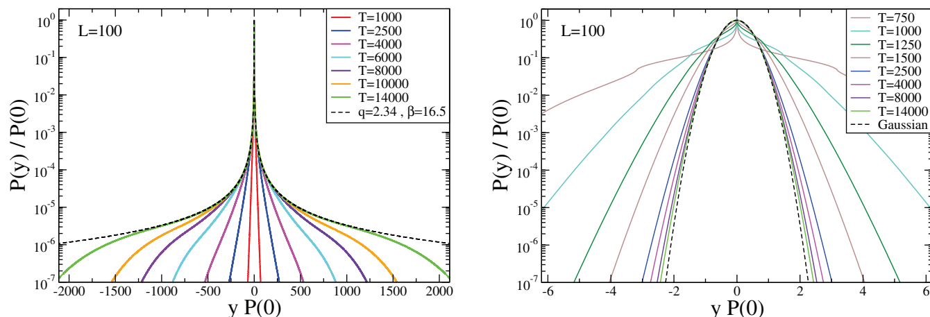
Fig. 7: (Colour on-line) Comparison of the T dependence for fixed values of L with p = 5 \cdot 10^{-6} for the correlated (left panel) and the uncorrelated (right panel) P(y, T) distribution (see text for the details).
