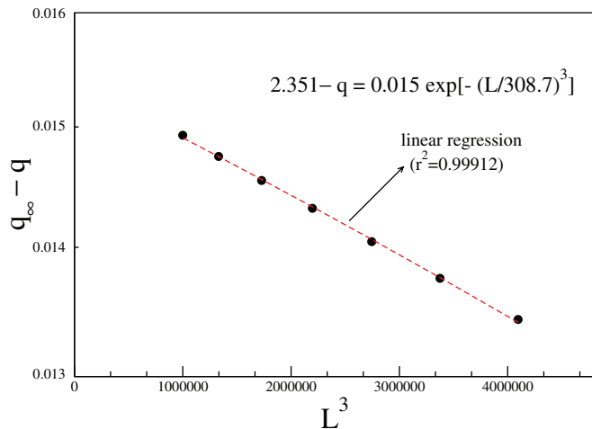
Fig. 5: (Colour on-line) Linear-log representation for the L dependence of q values. This exponential dependence suggests an asymptotic value around q_\infty \simeq 2.351 .
