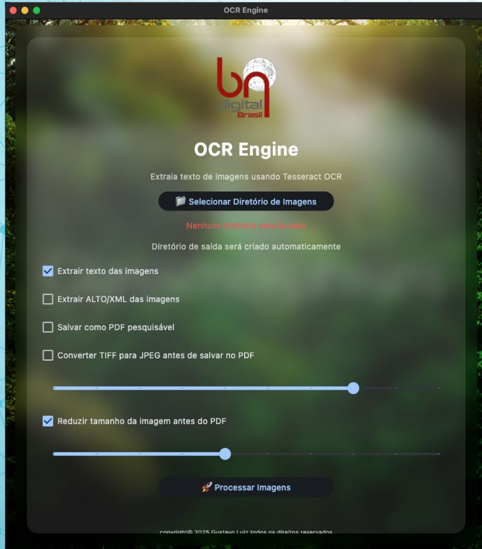
OCR ENGINE
