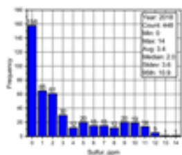
Figure 12. Sulfur content for biodiesel samples, January-December 2018
