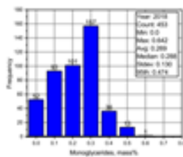
Figure 11. Monoglyceride content for biodiesel samples, January-December 2018
