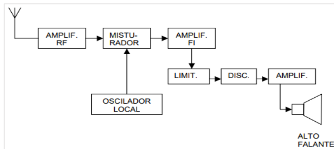
Diagrama de blocos Receptor FM
