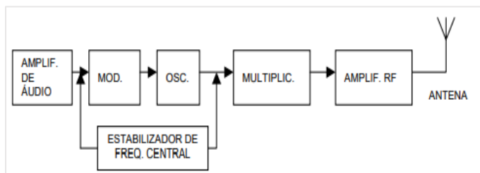
Diagrama de blocos Transmissor FM
