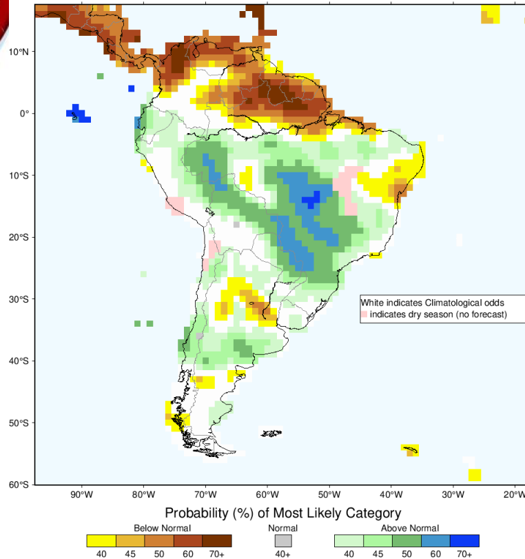
IRI Multi-Model Probability Forecast for Precipitation for June-July-August 2026, Issued May 2026
