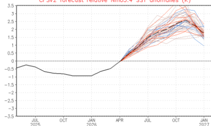
CFSv2 forecast relative Nino3.4 SST anomalies (K)
