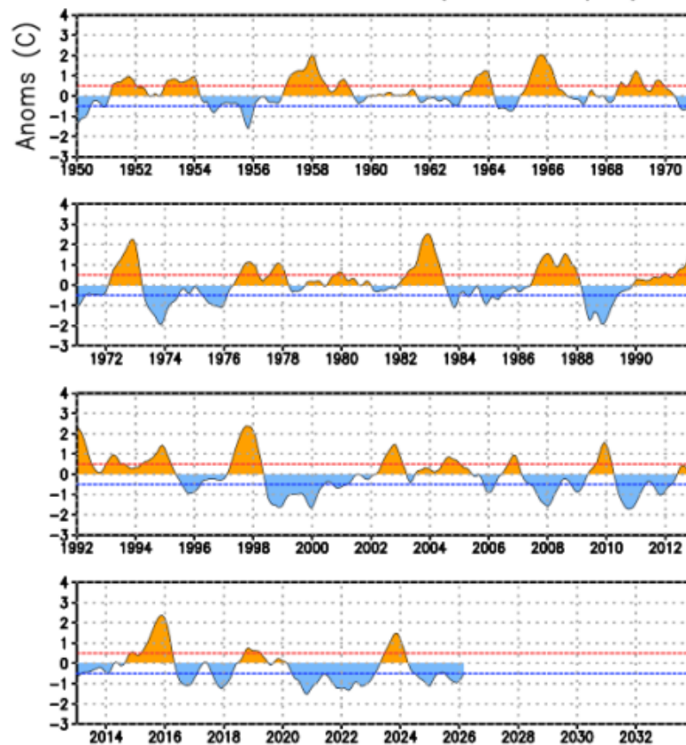
Relative Oceanic Nino Index (ERSST.v5 RONI) 3mrm Relative Nino 3.4 SST Anomalies (1991-2020 base period)
