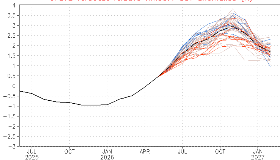
CFSv2 forecast relative Nino3.4 SST anomalies (K)
