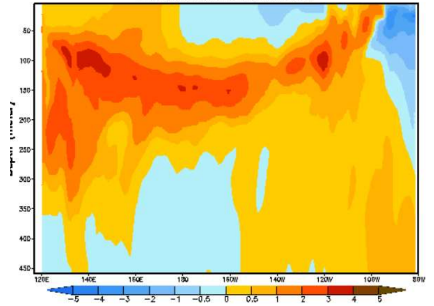
Equatorial Temperature Anomaly (°C) Pentad centered on 23 JAN 2026
