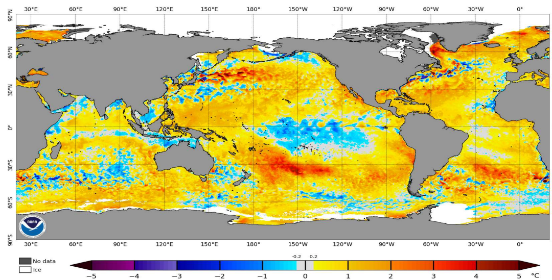
NOAA Coral Reef Watch Daily 5km SST Anomalies (v3.1) 26 Jan 2026
