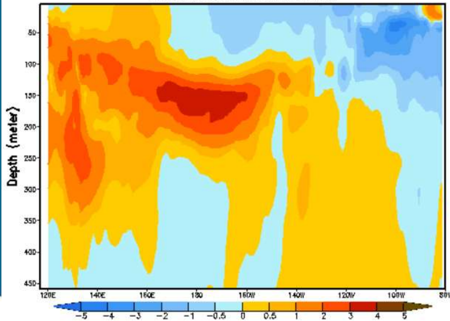
Equatorial Temperature Anomaly (°C) Pentad centered on 19 DEC 2025
