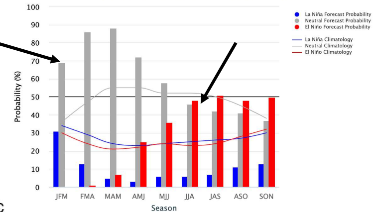
Mid-January 2026 IRI Model-Based Probabilistic ENSO Forecasts
