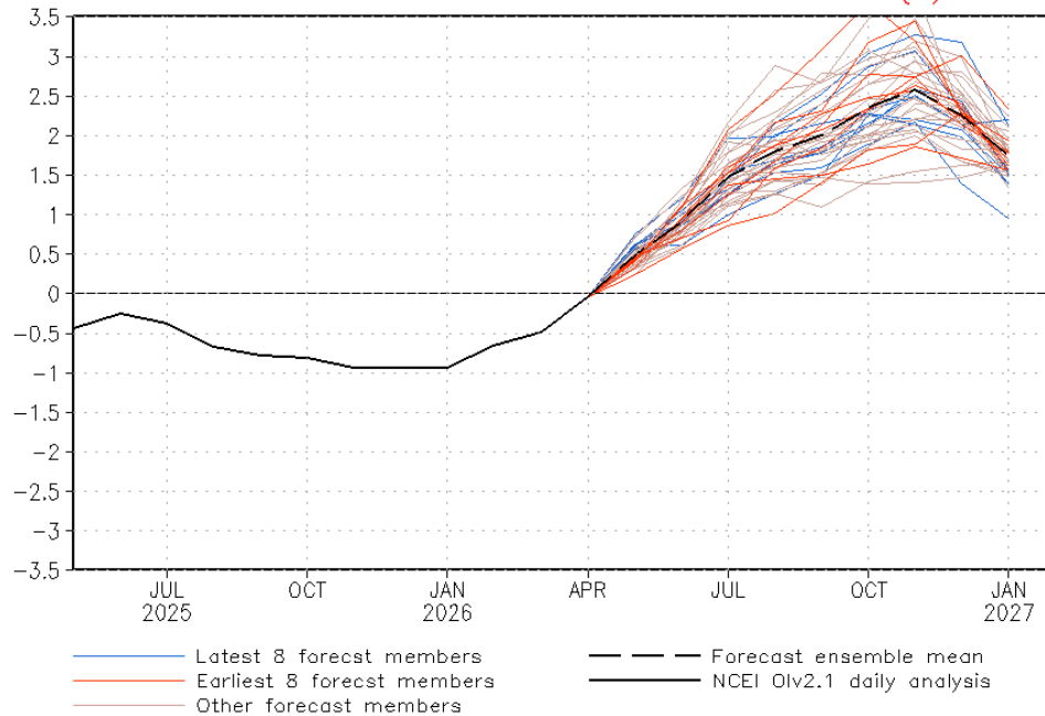
CFSv2 forecast relative Nino3.4 SST anomalies (K)
