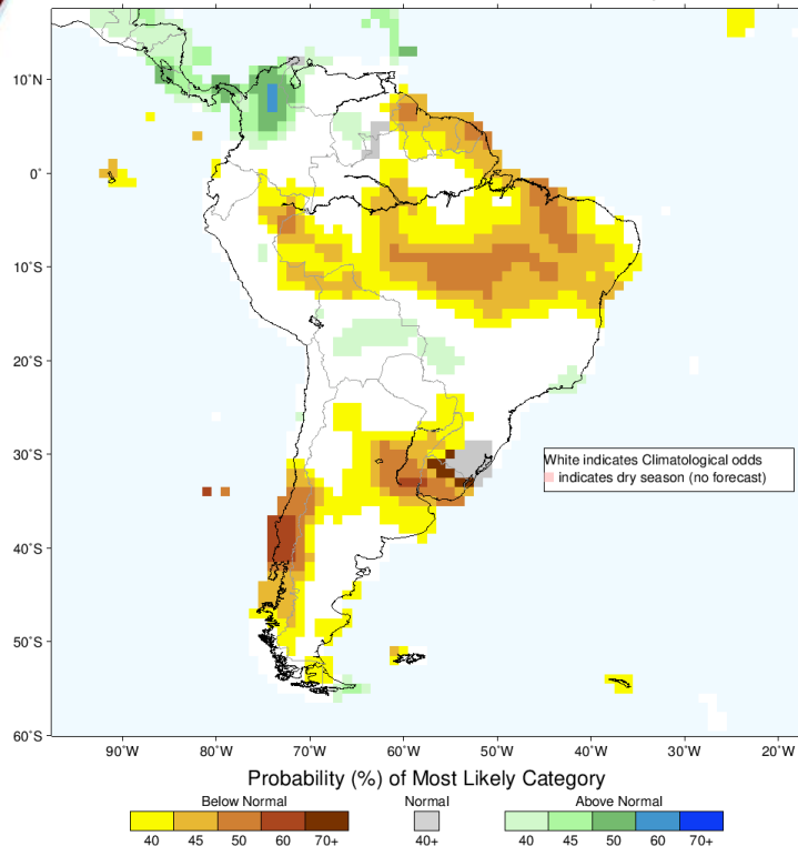
IRI Multi-Model Probability Forecast for Precipitation for October–November–December 2024, Issued July 2024
