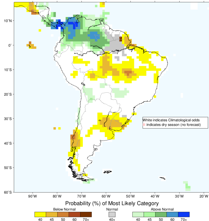
IRI Multi-Model Probability Forecast for Precipitation for November–December–January 2025, Issued July 2024
