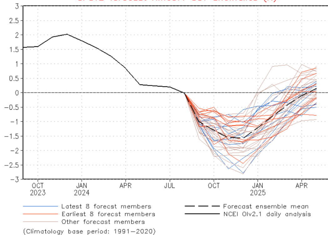
CFSv2 forecast Nino3.4 SST anomalies (K)
