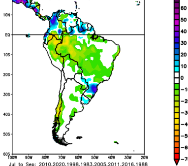
GPCC Precipitation V2020 Combined Precipitation (mm) Composite Anomaly 1991-2020 clima
