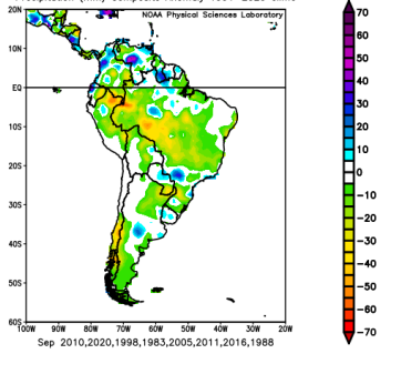
GPCC Precipitation V2020 Combined Precipitation (mm) Composite Anomaly 1991-2020 clima
