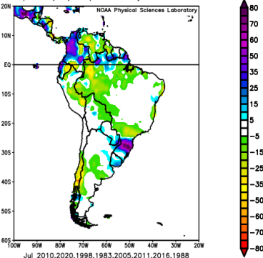
GPCC Precipitation V2020 Combined Precipitation (mm) Composite Anomaly 1991-2020 clima
