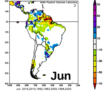
GPCC Precipitation V2020 Combined Precipitation (mm) Composite Anomaly 1991-2020 clima
