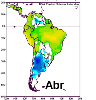
U of Delaware V5.01 Surface Air Temperature (C) Composite Anomaly
