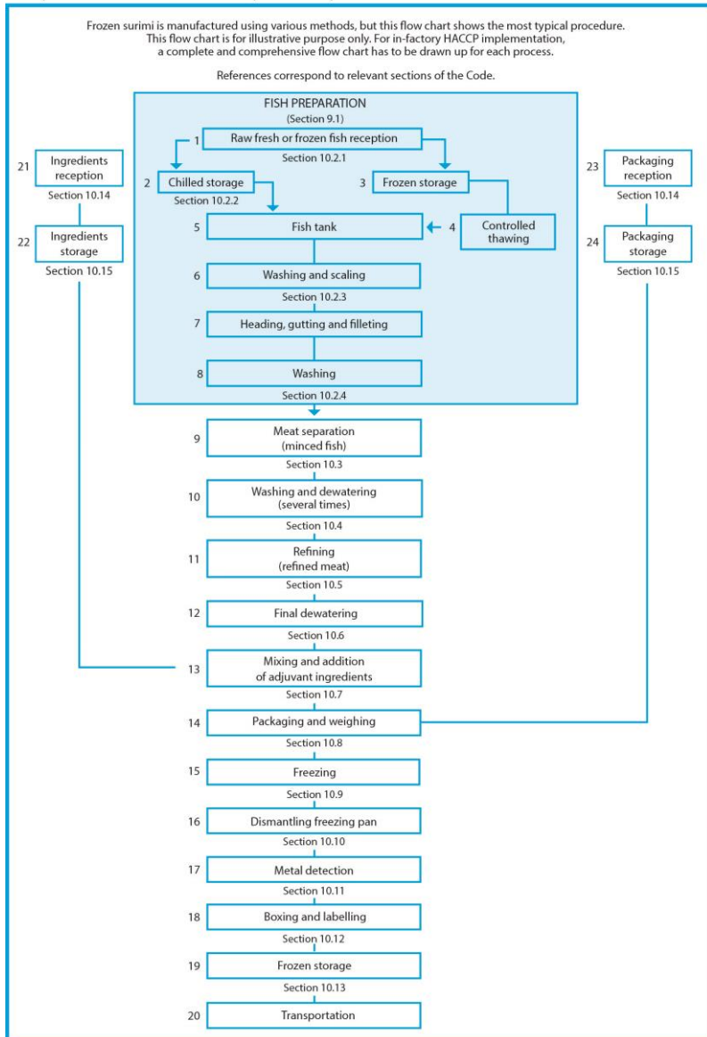
Figure 10.1 Example flow chart of a frozen surimi-production process
