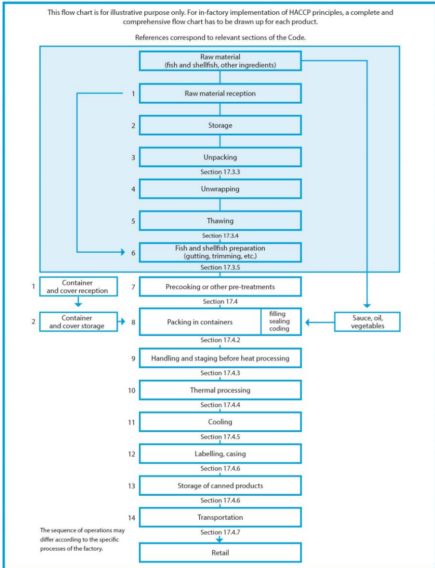
Figure 17.1 Example flow chart for the processing of canned fish and shellfish
