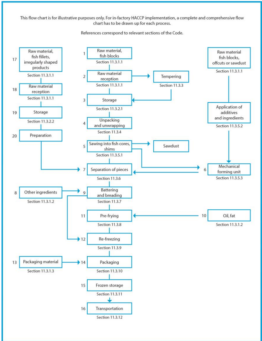
Figure 11.1 Example flow chart for the processing of coated fish products
