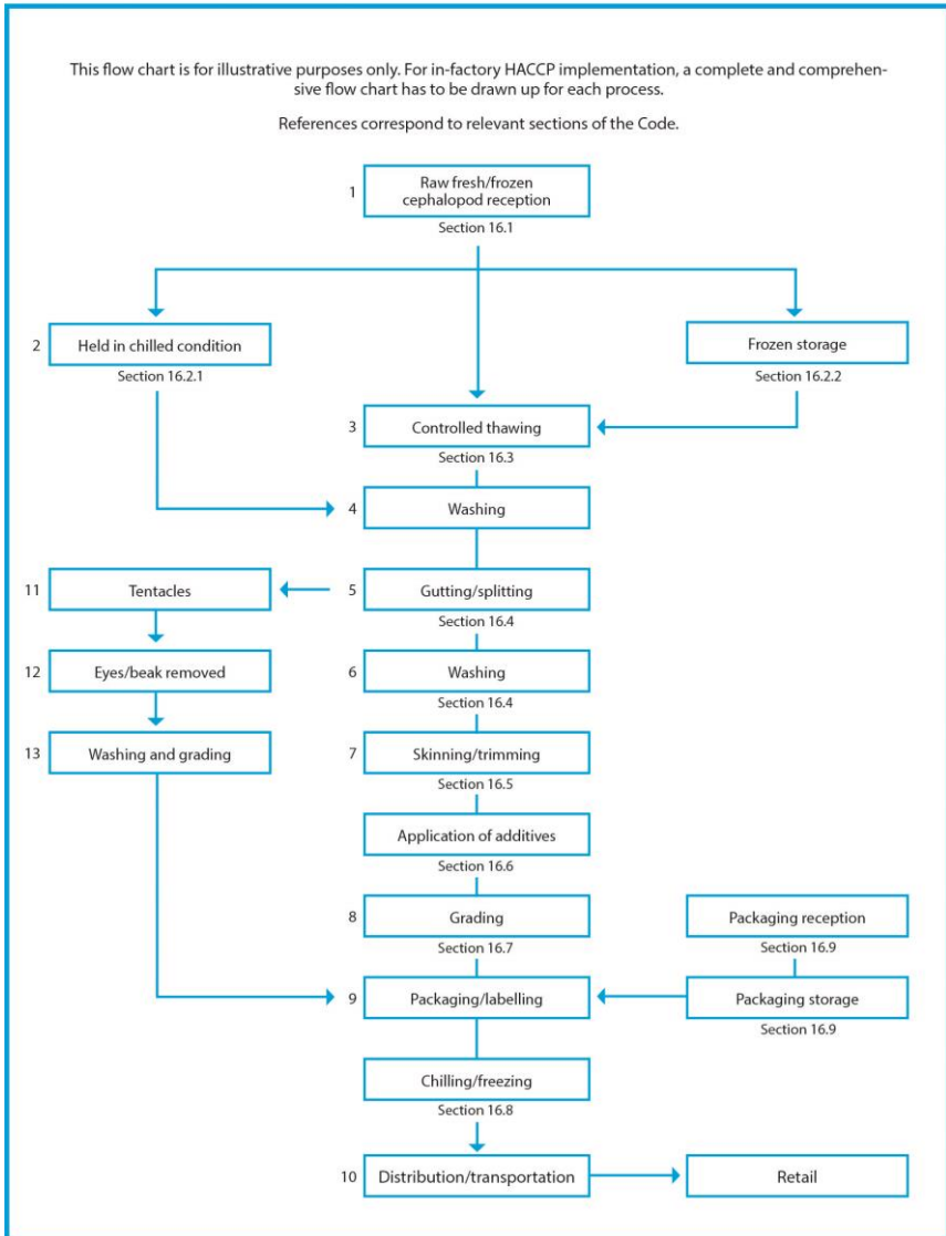
Figure 16.1 Example of a possible squid processing line
