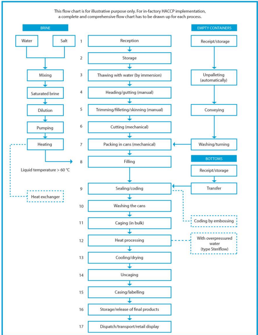
Figure 5.2 Example flow chart for a canned tuna fish in brine-processing line
