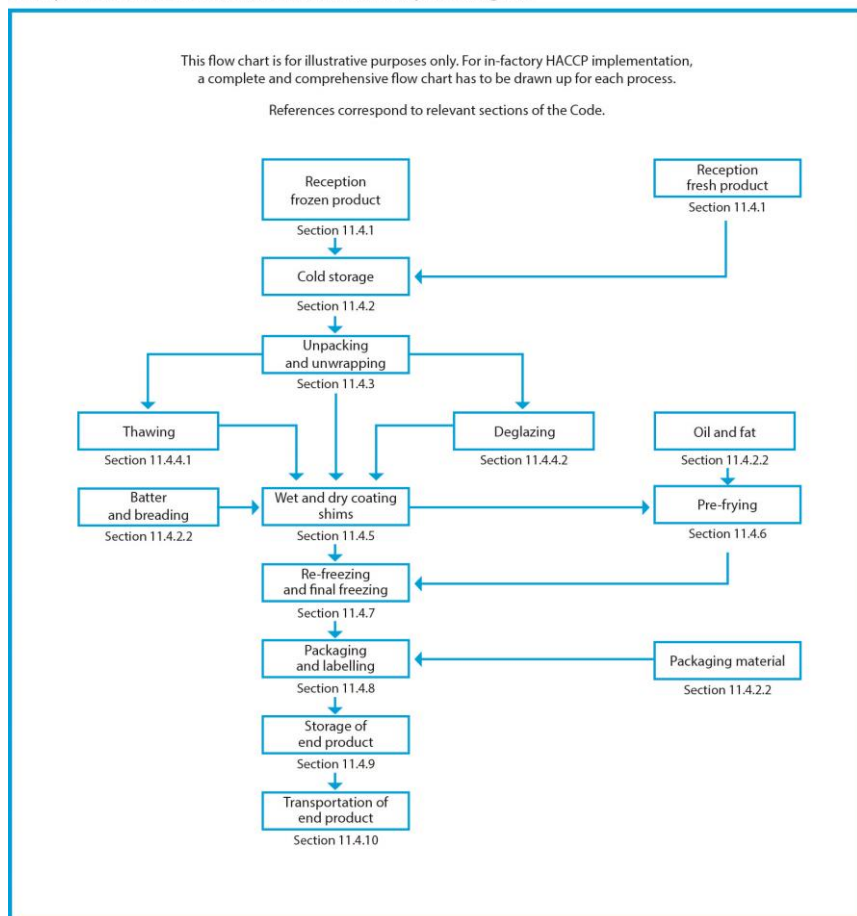
Figure 11.2 Example flow chart of a coated molluscan shellfish-processing line
