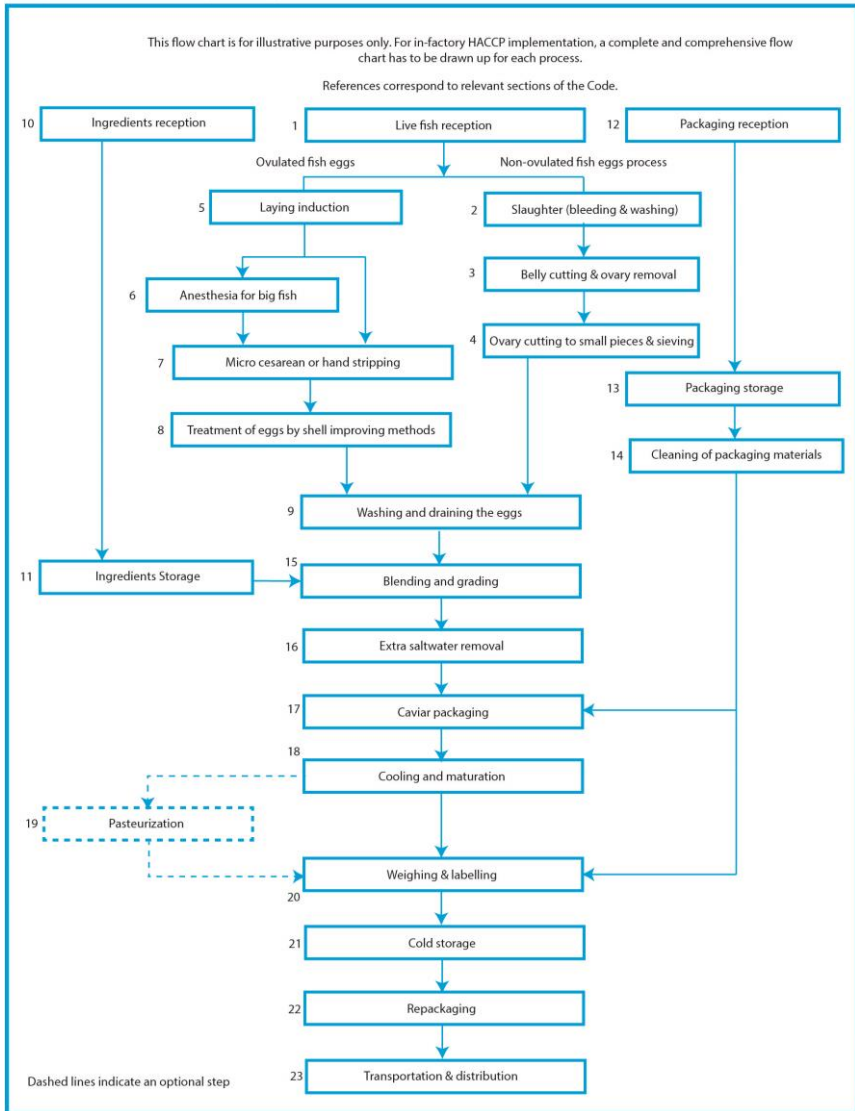
Figure 19.1 Example flow chart for caviar processing
