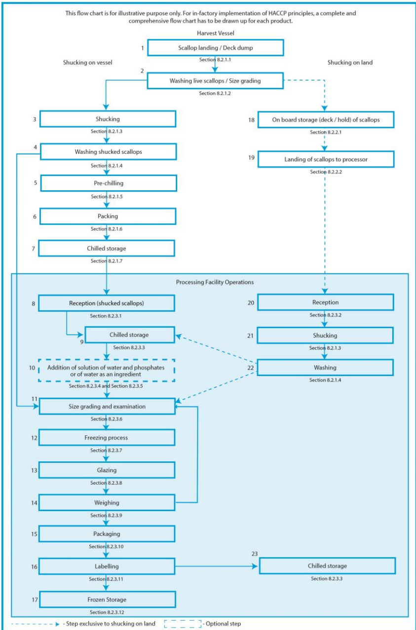
Figure 8.1 Example flow chart for the production of scallop product
