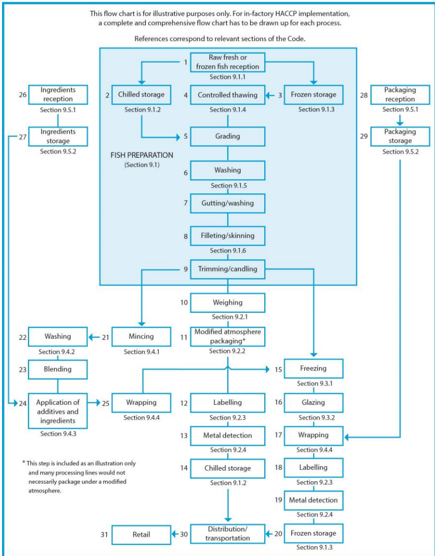
Figure 9.1 Example flow chart of a fish fillet-preparation line, including MAP, mincing and freezing operations
