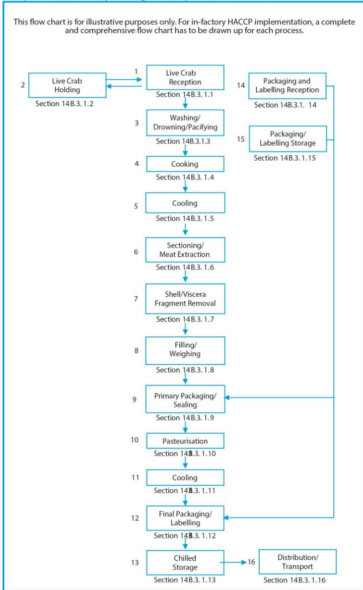
Figure 14B.1 Example flow chart for the processing of chilled pasteurized crabmeat
