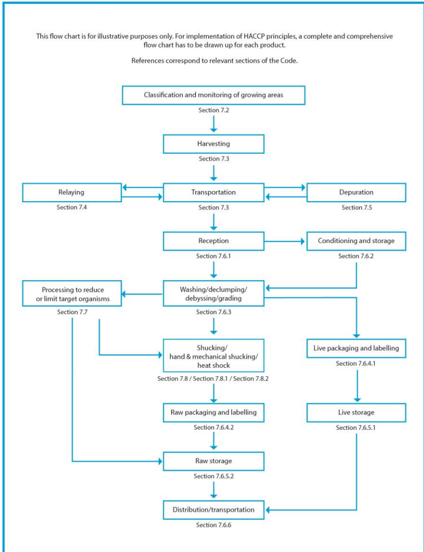
Figure 7.1 Example flow chart for the production of live and raw bivalve molluscs
