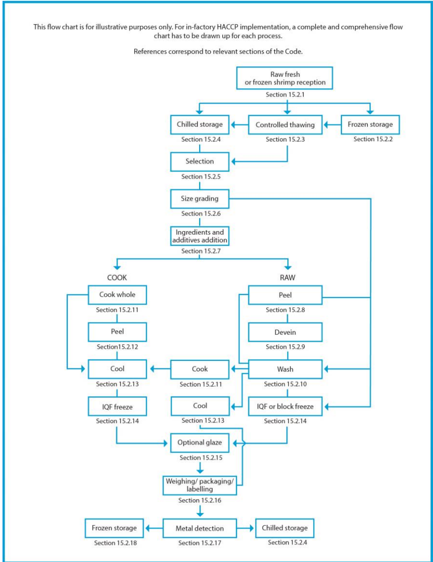
Figure 15.1 Example flow chart of a shrimp and prawn processing line
