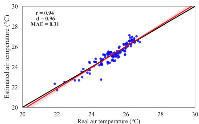
Fig. 4 Statistical determination to estimate the mean air temperature (°C) in the Midwest region of Brazil. r is correlation coefficients, d is Willmott agreement, MAE is mean absolute error
