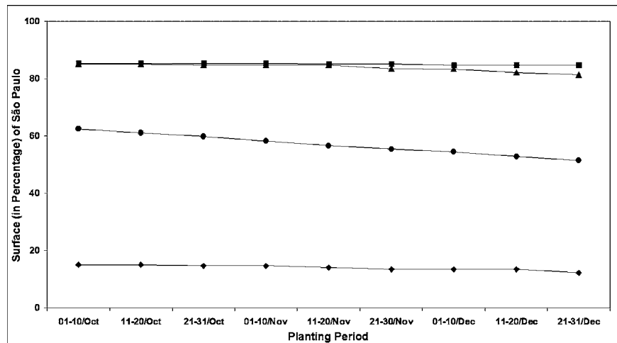
Figure 8. Surface (in percentage) of São Paulo suitable for early cultivars of corn, in soils of medium water holding capacity (50 mm), planted from October to December, in four climate scenarios. ◆, Increase of 5.8°C in Temperature and 15% in Precipitation; ●, Increase of 3°C in Temperature and 15% in Precipitation; ▲, Increase of 1°C in Temperature and 15% in Precipitation; ■, Current Situation.
