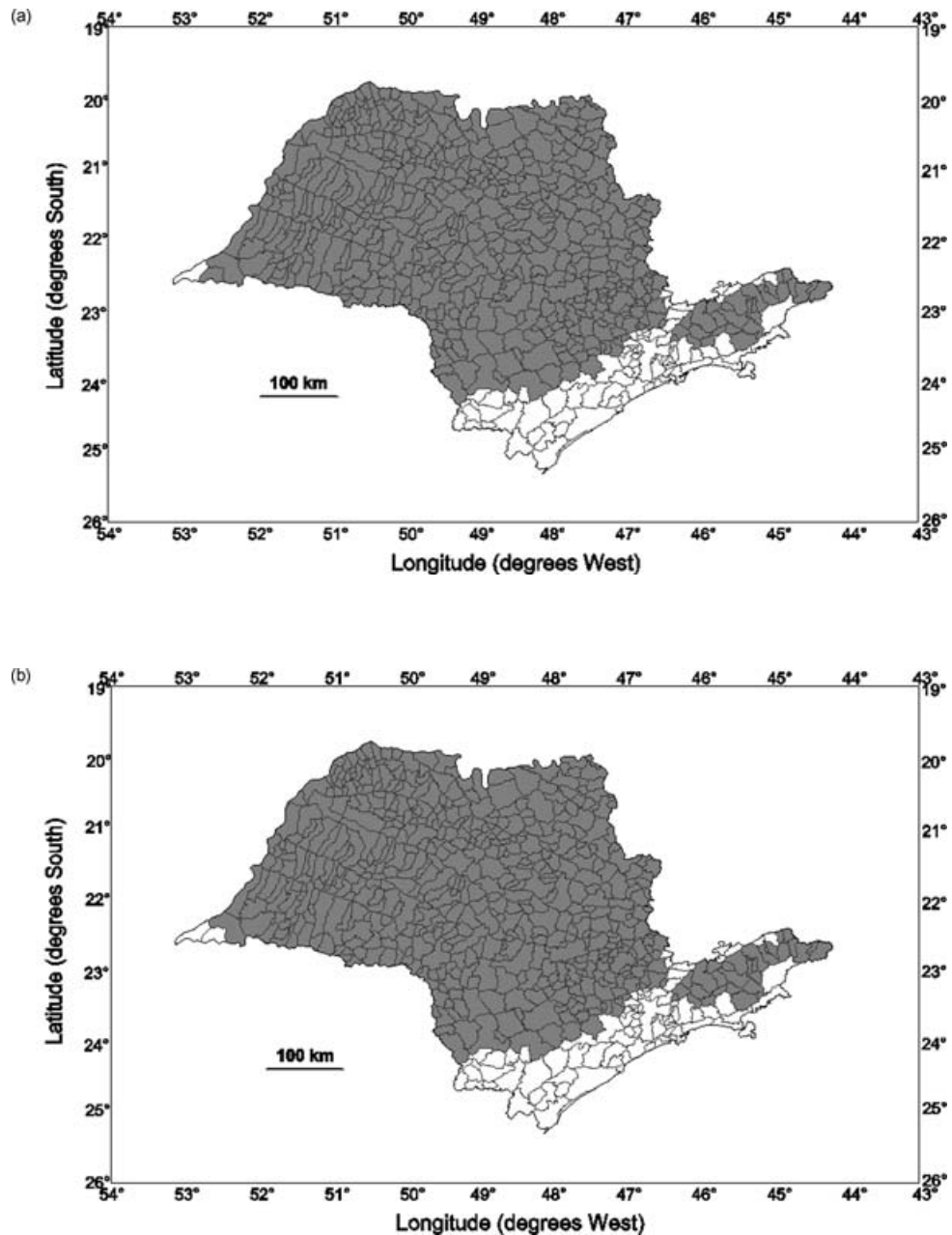
Figure 6. Suitable (grey) and unsuitable (white) areas for early cultivars of corn, planted from November 11 to 20, in the state of São Paulo, Brazil, in soils of medium water holding capacity (50 mm) considering: (a) the current climate situation, (b) an increase of 15% in precipitation and 1°C in temperature, (c) an increase of 15% in precipitation and 3°C in temperature, and (d) an increase of 15% in precipitation and 5.8°C in temperature, above the current values of precipitation and temperature.
