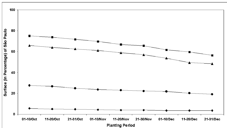
Figure 7. Surface (in percentage) of São Paulo suitable for early cultivars of corn, in soils of low water holding capacity (30 mm), planted from October to December, in four climate scenarios. —◆, Increase of 5.8°C in Temperature and 15% in Precipitation; —●, Increase of 3°C in Temperature and 15% in Precipitation; —▲, Increase of 1°C in Temperature and 15% in Precipitation; —■, Current Situation.
