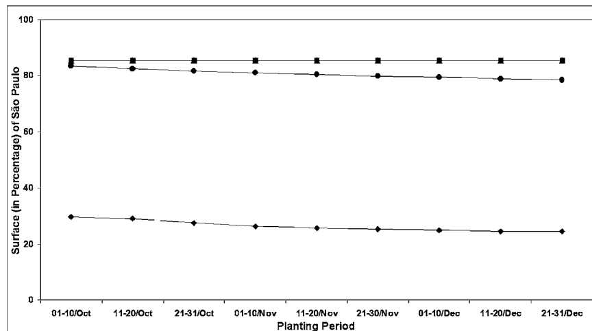
Figure 9. Surface (in percentage) of São Paulo suitable for early cultivars of corn, in soils of high water holding capacity (70 mm), planted from October to December, in four climate scenarios. ◆, Increase of 5.8°C in Temperature and 15% in Precipitation; ●, Increase of 3°C in Temperature and 15% in Precipitation; ▲, Increase of 1°C in Temperature and 15% in Precipitation; ■, Current Situation.
