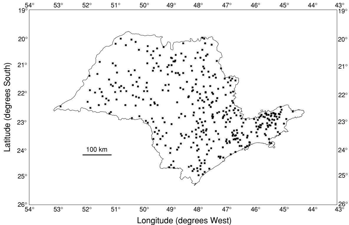
Figure 1. Rainfall network with 390 ground stations located in the state of São Paulo (Brazil) having data from 1961 to 1990, used in agricultural zoning.
