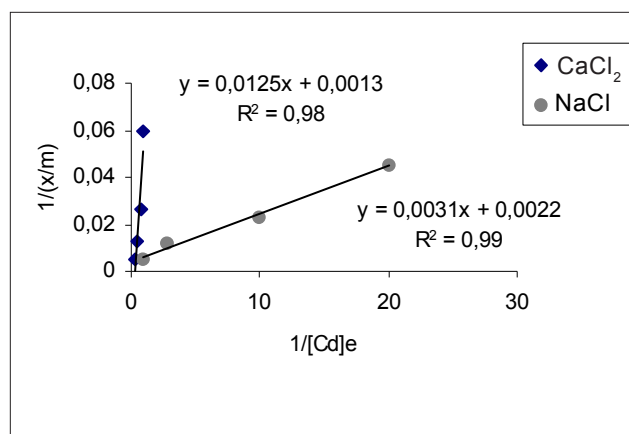
Figure 6 - Langmuir's adsorption isotherm of cadmium in Zone 3.
