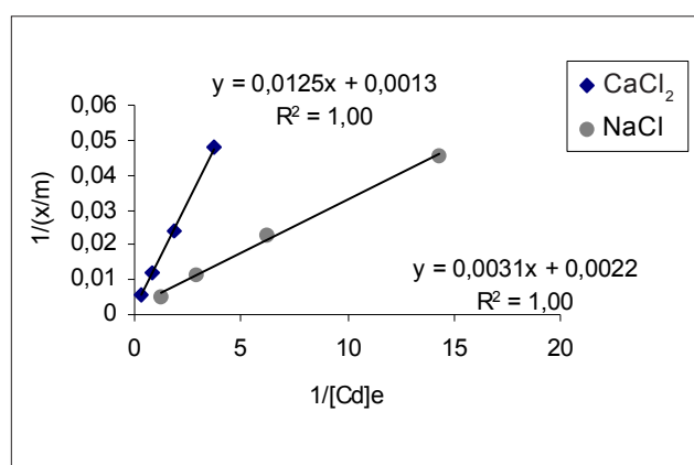
Figure 5 - Langmuir's adsorption isotherm of cadmium in Zone 2.
