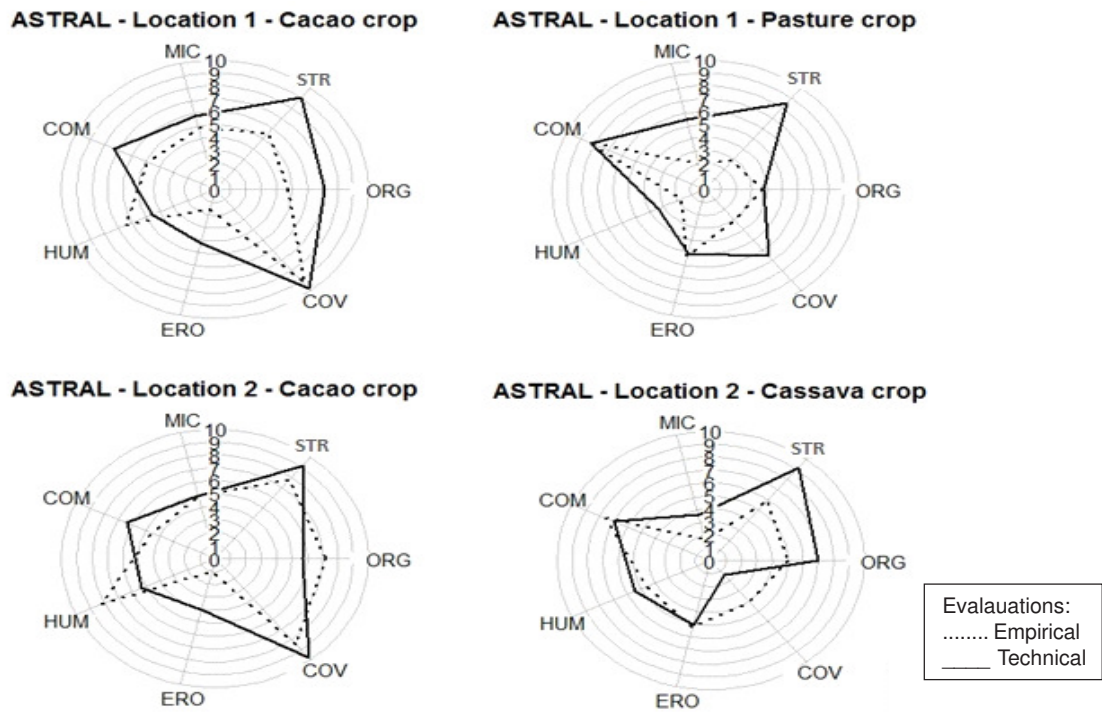
Figure 2. Radial charts of the soil quality indicators for empirical and technical evaluations at ASTRAL settlement. ORG: organic matter; COV: soil cover; ERO: erosion; HUM: humidity; COM: compaction; MIC: microbial activity; STR: structure.
