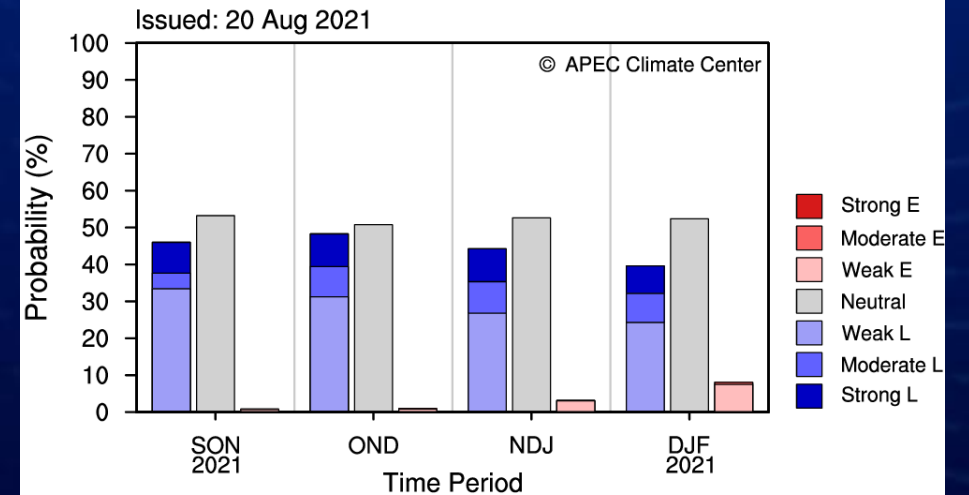
Probabilistic ENSO Forecast for 2021 SONDJF
